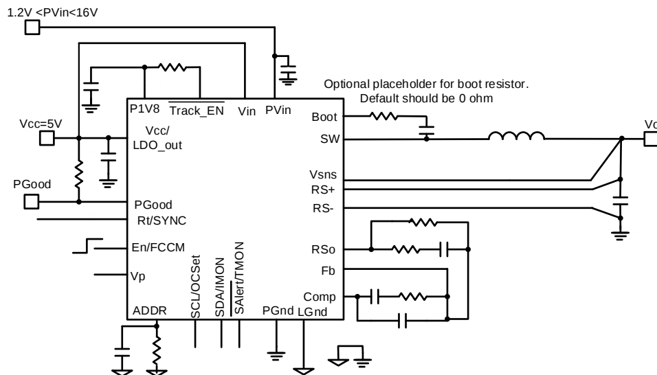
Figure 8: Using external V_{cc} , digital mode, V_o < 2.55V
