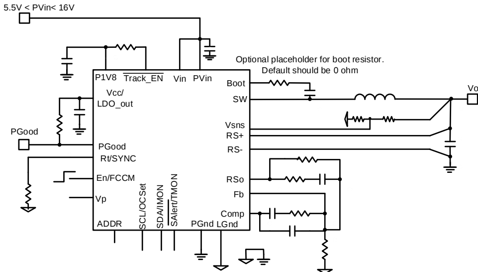
Figure 7: Using the internal LDO, analog mode, V_o < 2.55V
