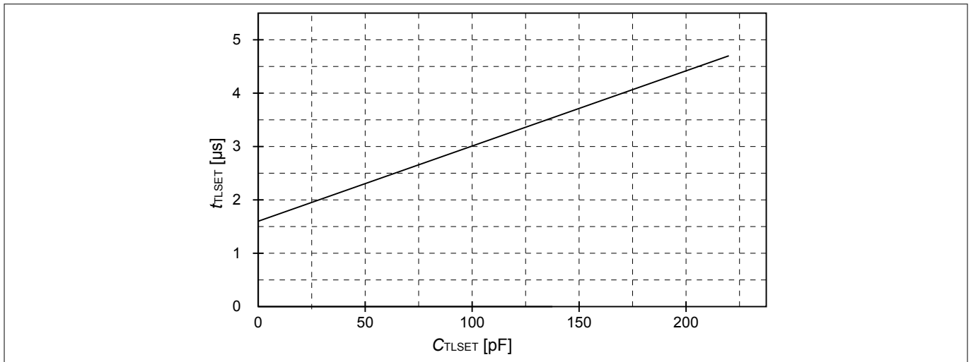
Figure 9 Typical t TLSET time over C TLSET capacitance
