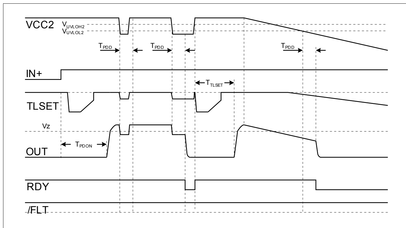
Figure 7-9 VCC2 Ramp Down and VCC2 Drop
