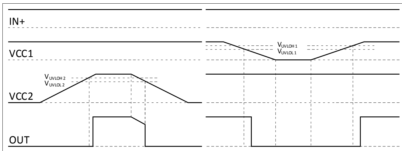
Figure 8 UVLO Behavior
