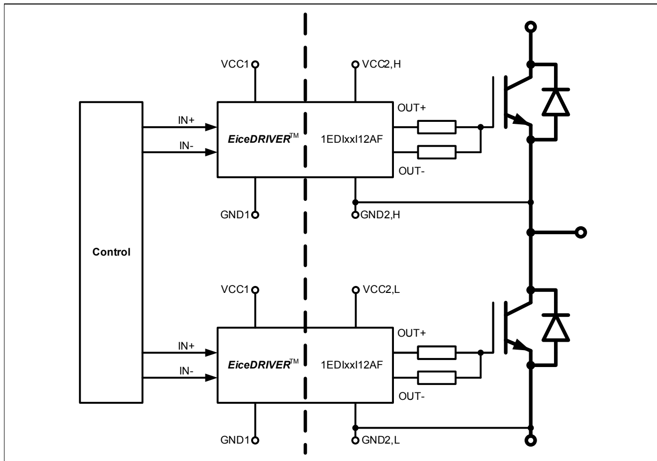
Figure 1 Typical Application
