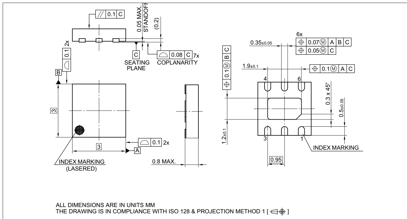
Figure 22 PG-WSON-6-1 outline dimensions
