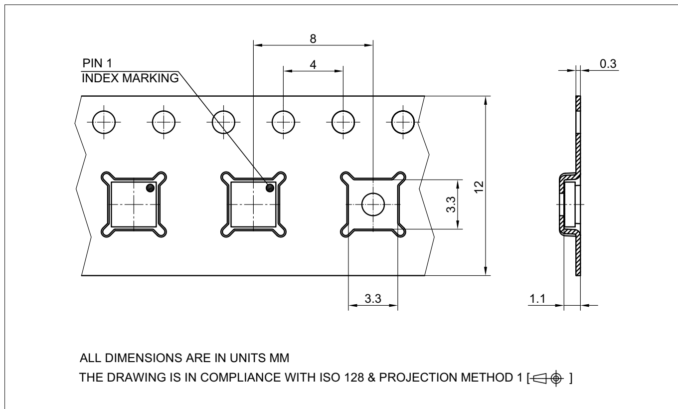
Figure 24 PG-WSO6-1 packaging dimensions
