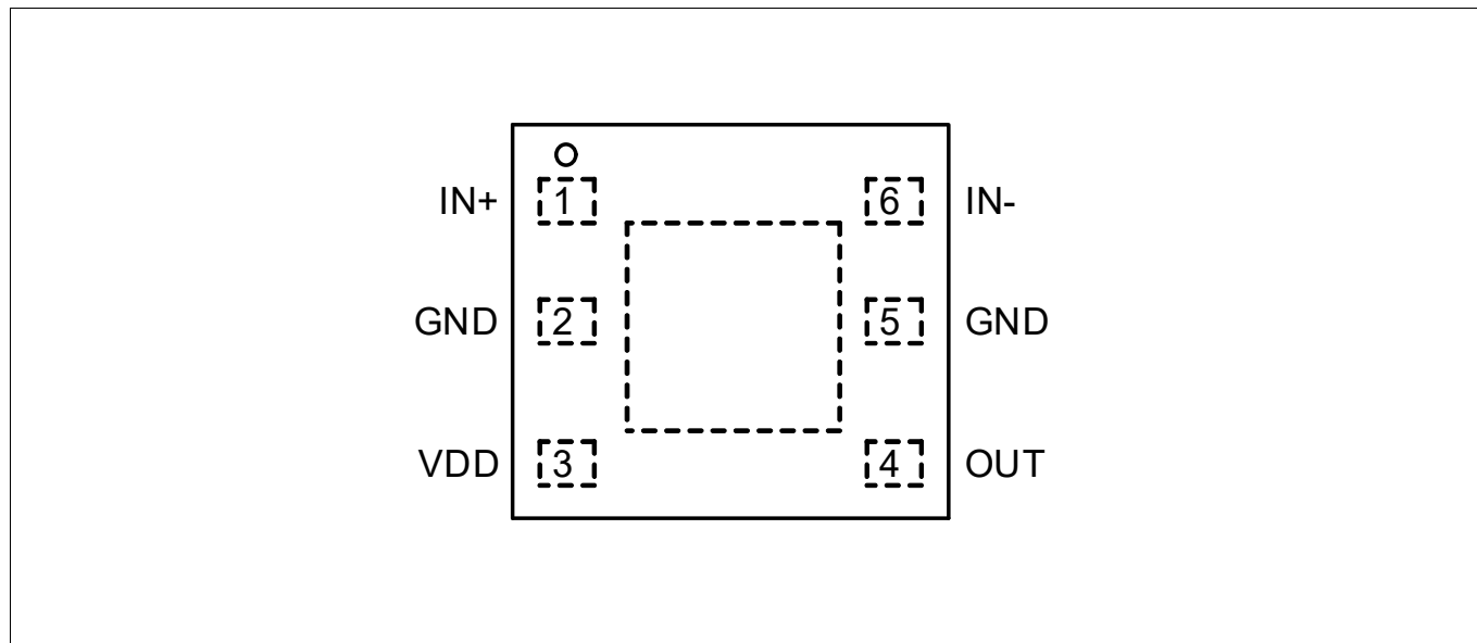
Figure 3 Pin configuration PG-WSO6-1 (top side view)
