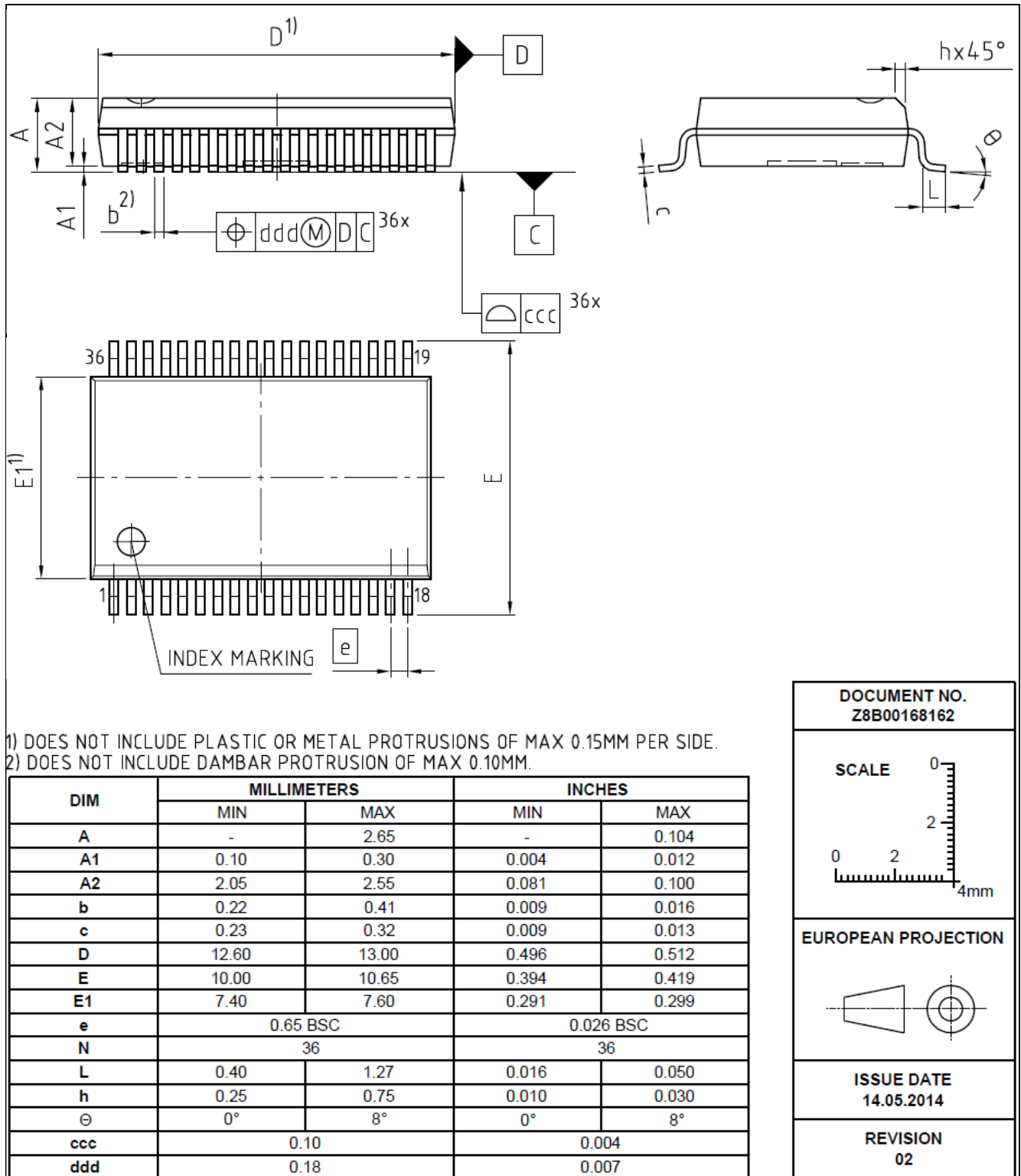
Figure 16 Package drawing
