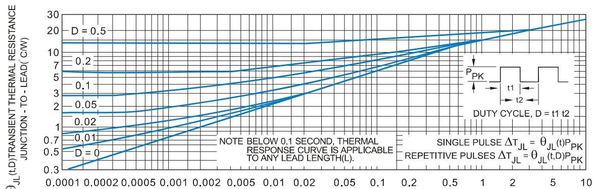
FIGURE 1. TYPICAL THERMAL RESPONSE L,
