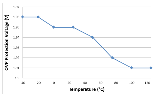
Fig.7 OVP Protection Voltage VS Temperature
