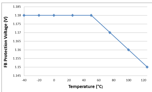
Fig.4 FB Protection Voltage VS Temperature
