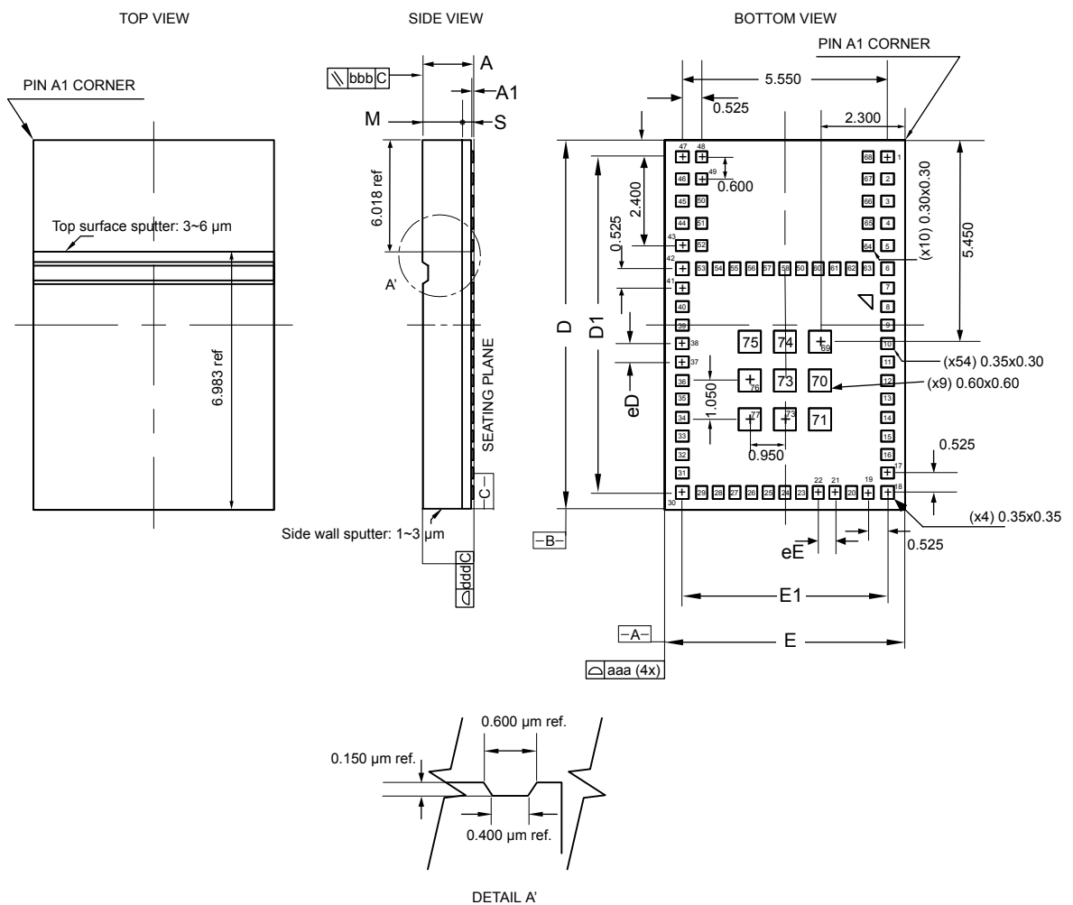
Figure 11. LGA77 - Outline
