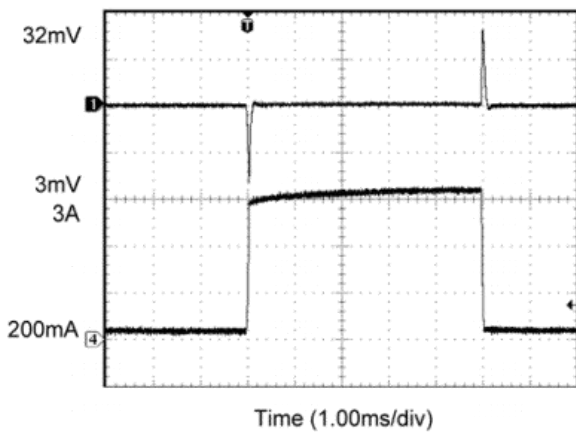
LM29302 Load Transient Response
