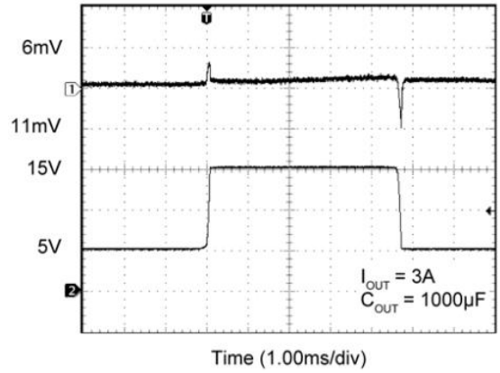
LM29302 Line Transient Response with 3A Load, 100µF Output Capacitance
