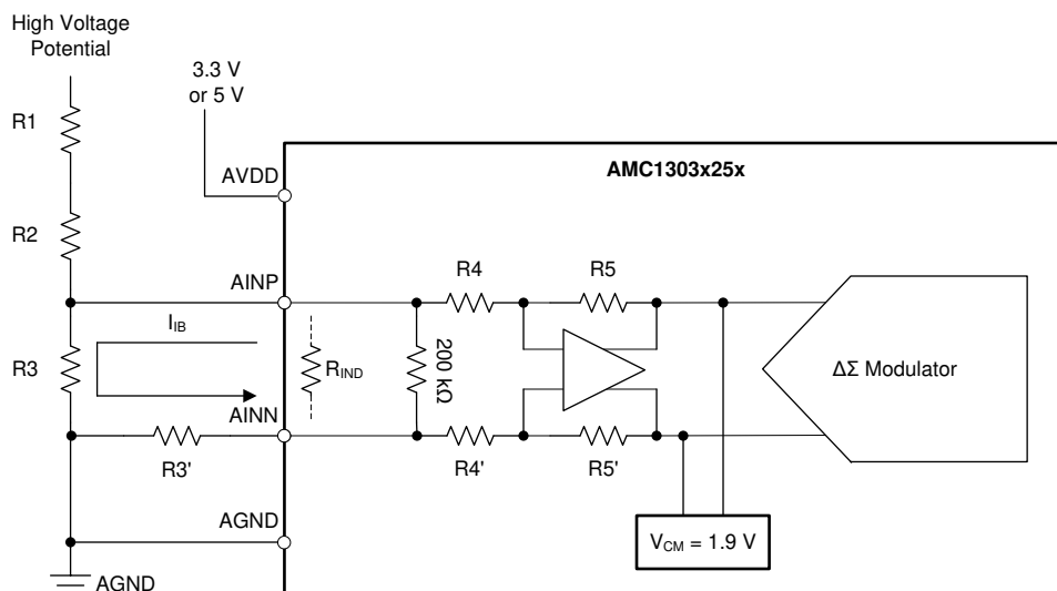
Figure 55. Using the AMC1303x25x for Isolated Voltage Sensing
