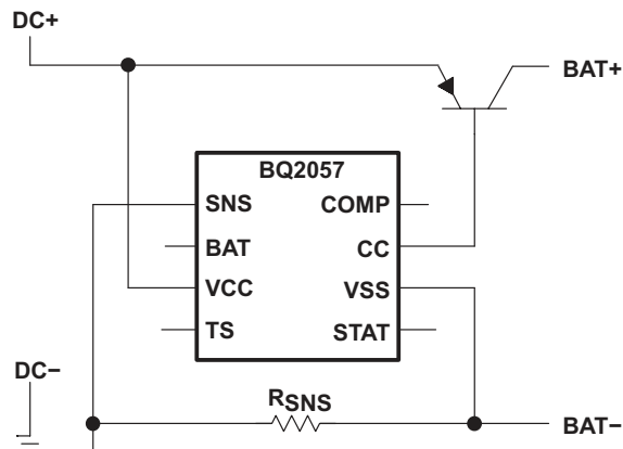
Figure 10-6. Low-Side Current Sensing
