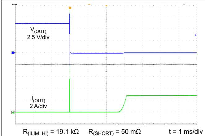
Figure 6-26. Hot Short
