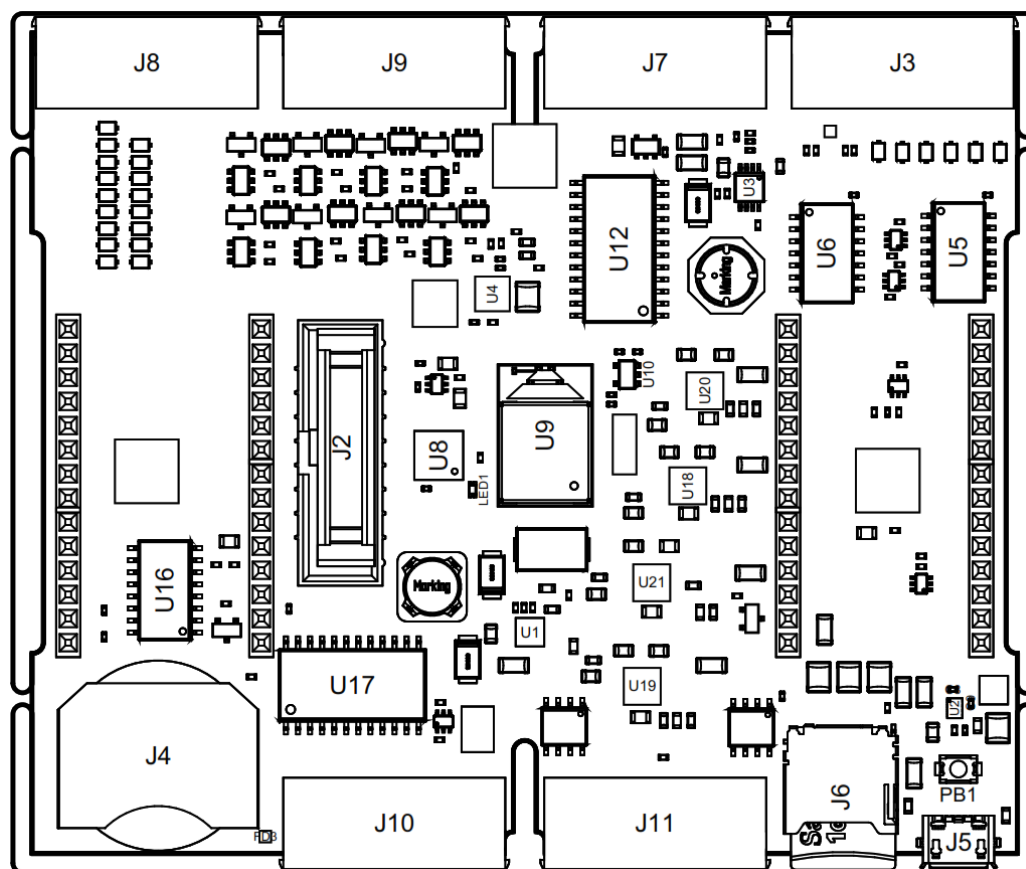
Board Topology
