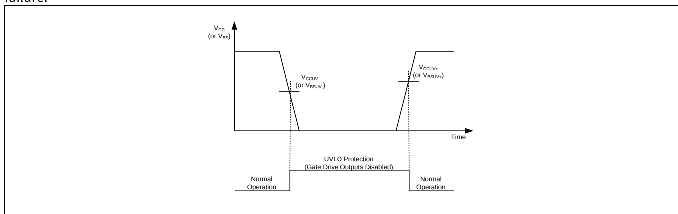
Figure 14 UVLO protection
