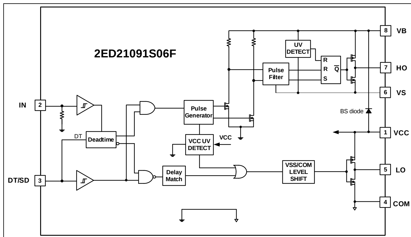
Figure 2 Block diagrams
