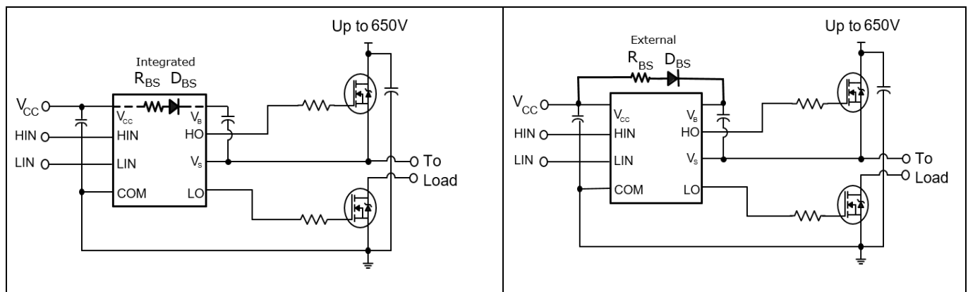
Figure 11 2ED218x with integrated components
