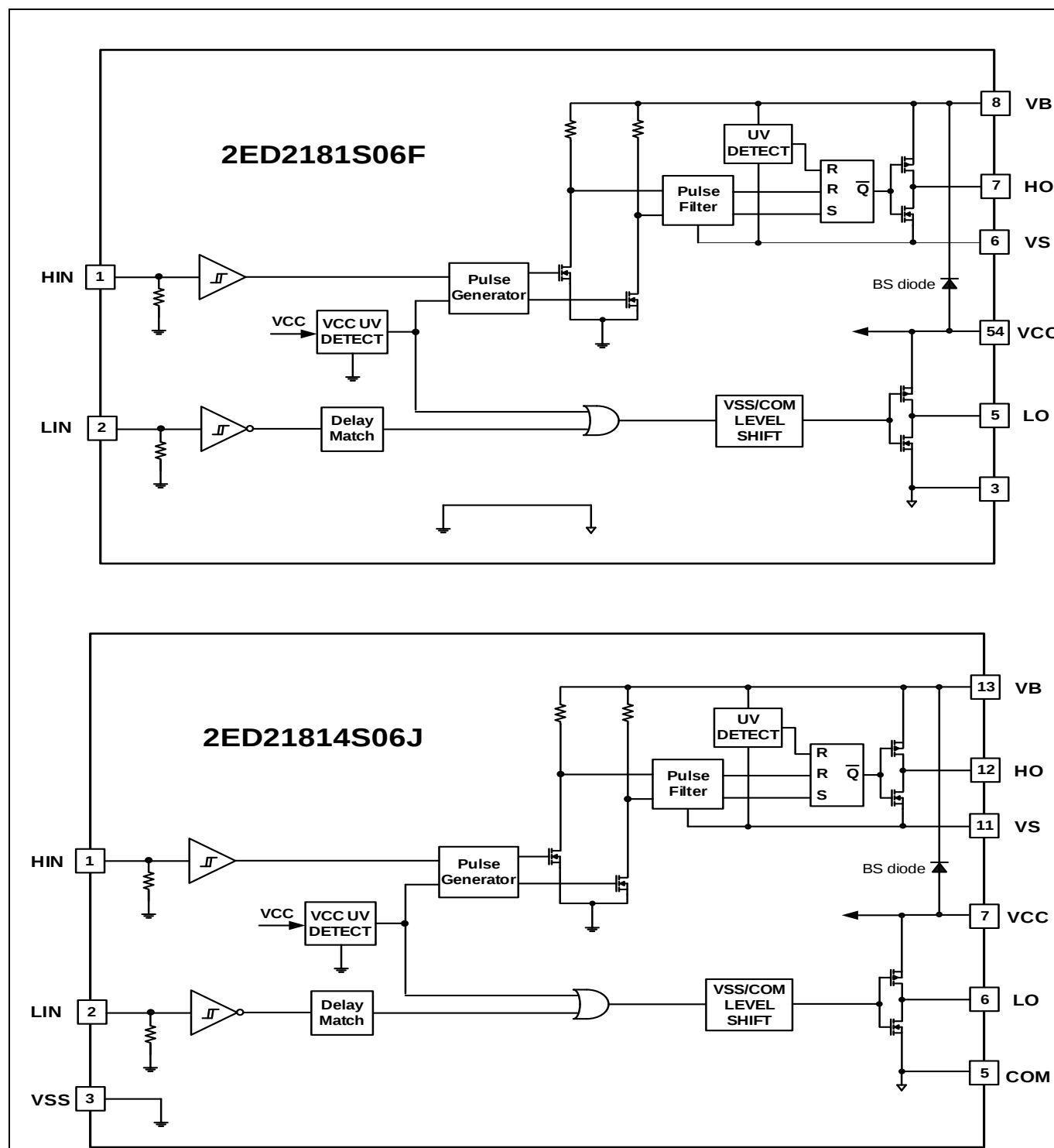
Figure 2 Block diagrams
