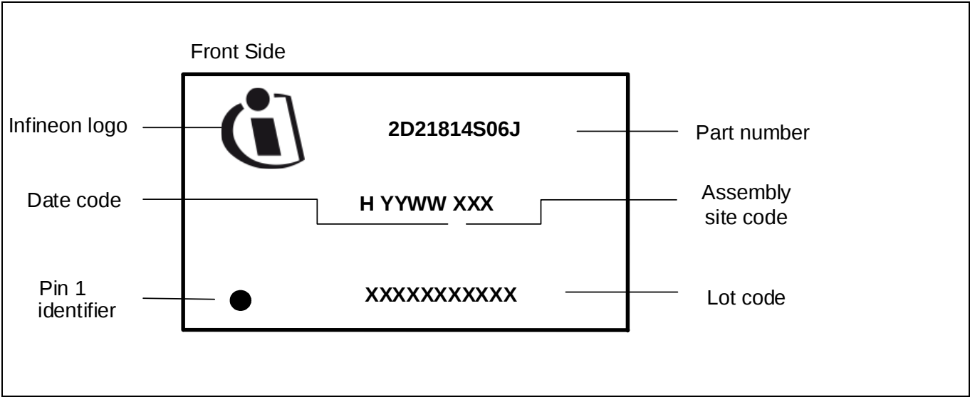
Figure 26 Marking information PG-DSO-14
