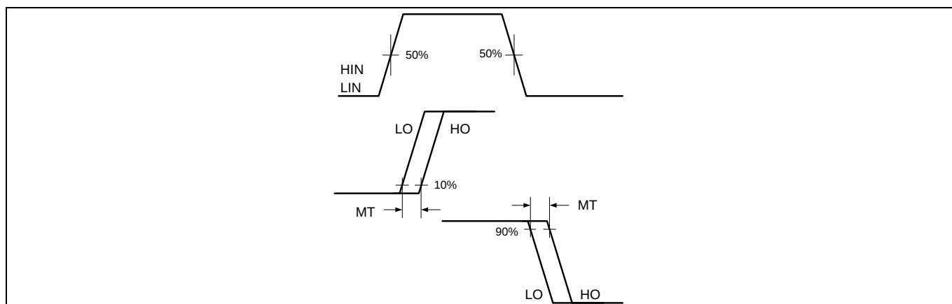
Figure 8 Delay matching waveform definition
