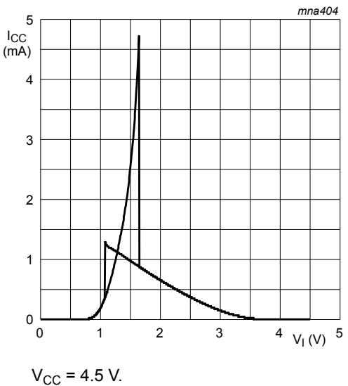
Fig. 12. Typical 74AHCT3G14-Q100 transfer characteristics
