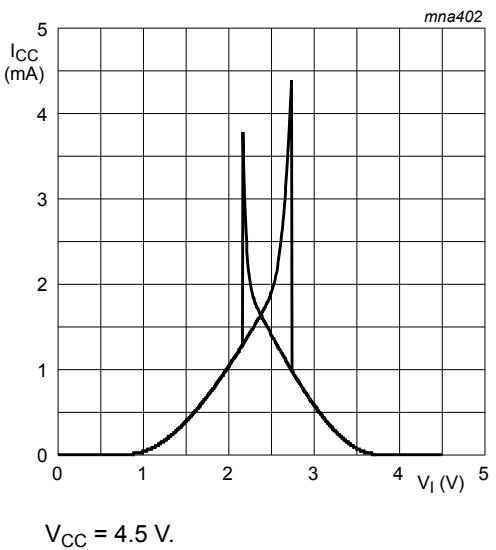
Fig. 10. Typical 74AHC3G14-Q100 transfer characteristics
