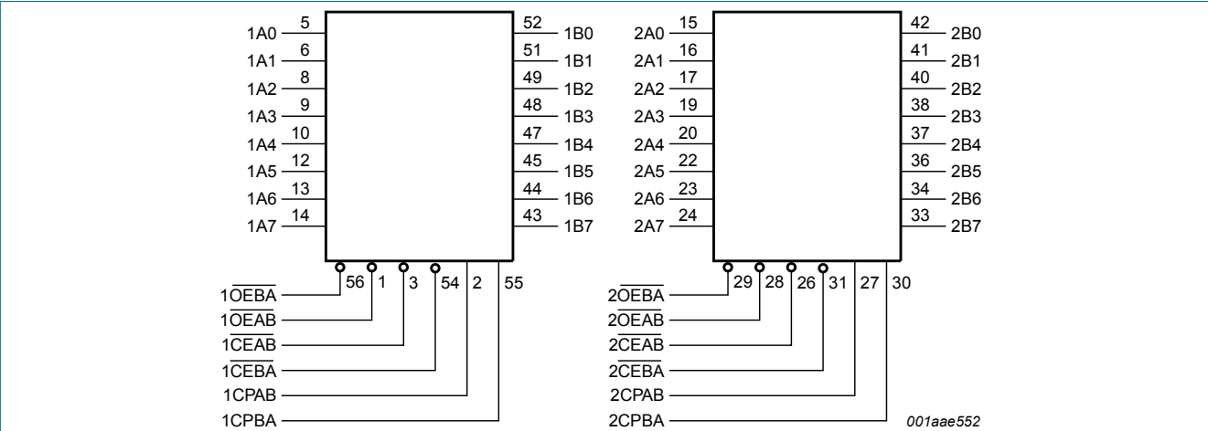
Figure 1. Logic symbol
