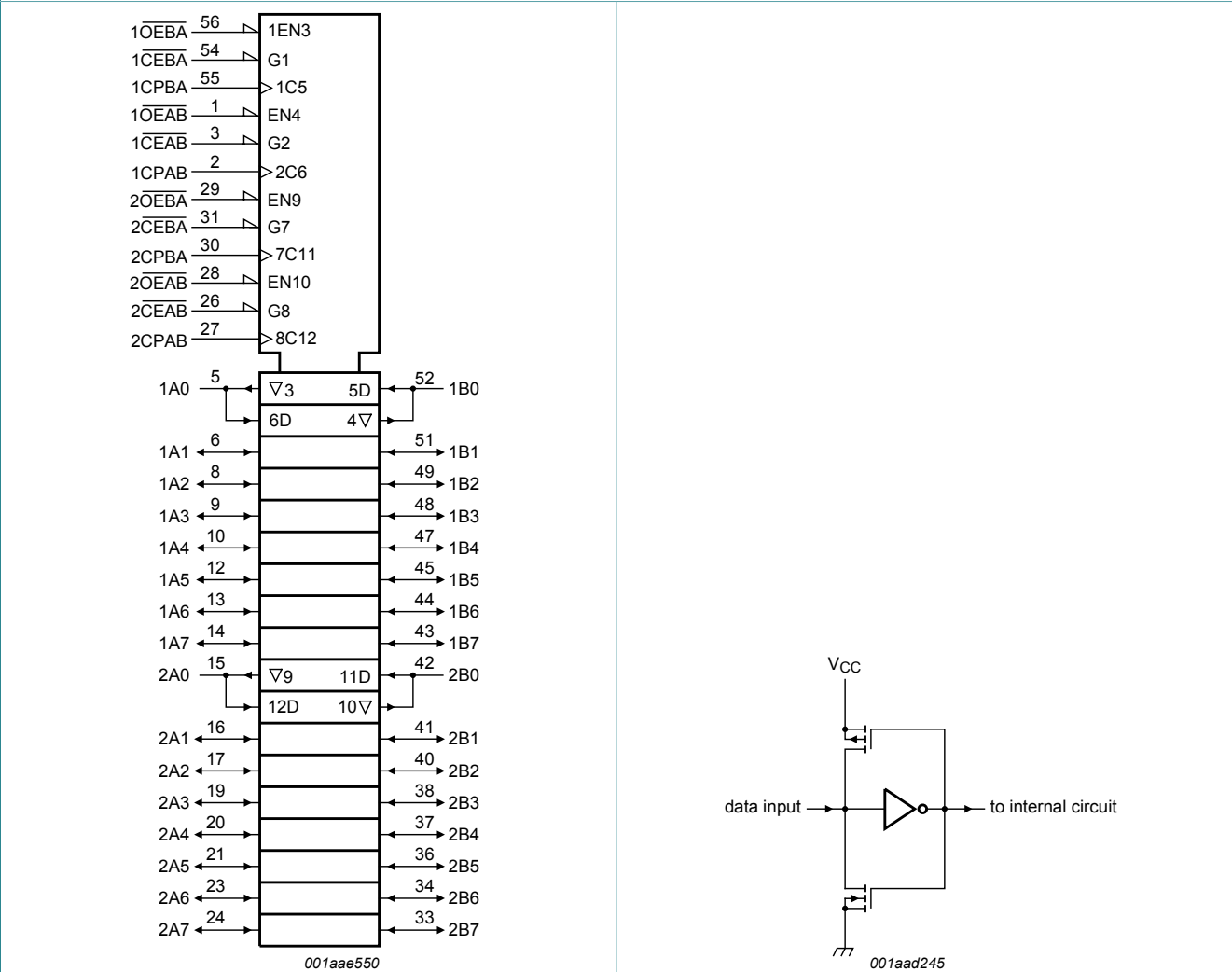
Figure 2. IEC logic symbol
