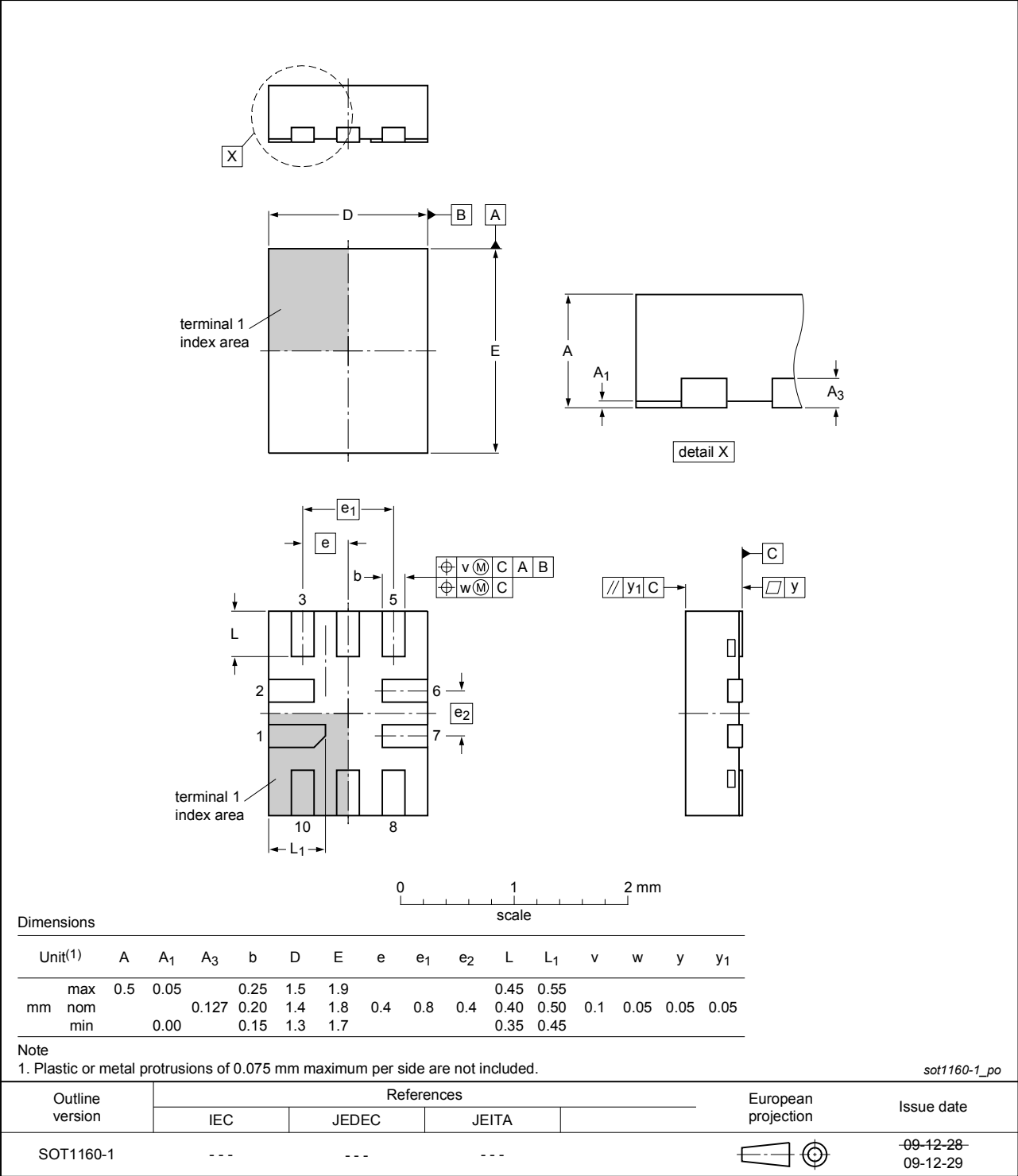
Figure 13. Package outline SOT1160-1 (XQFN10)
