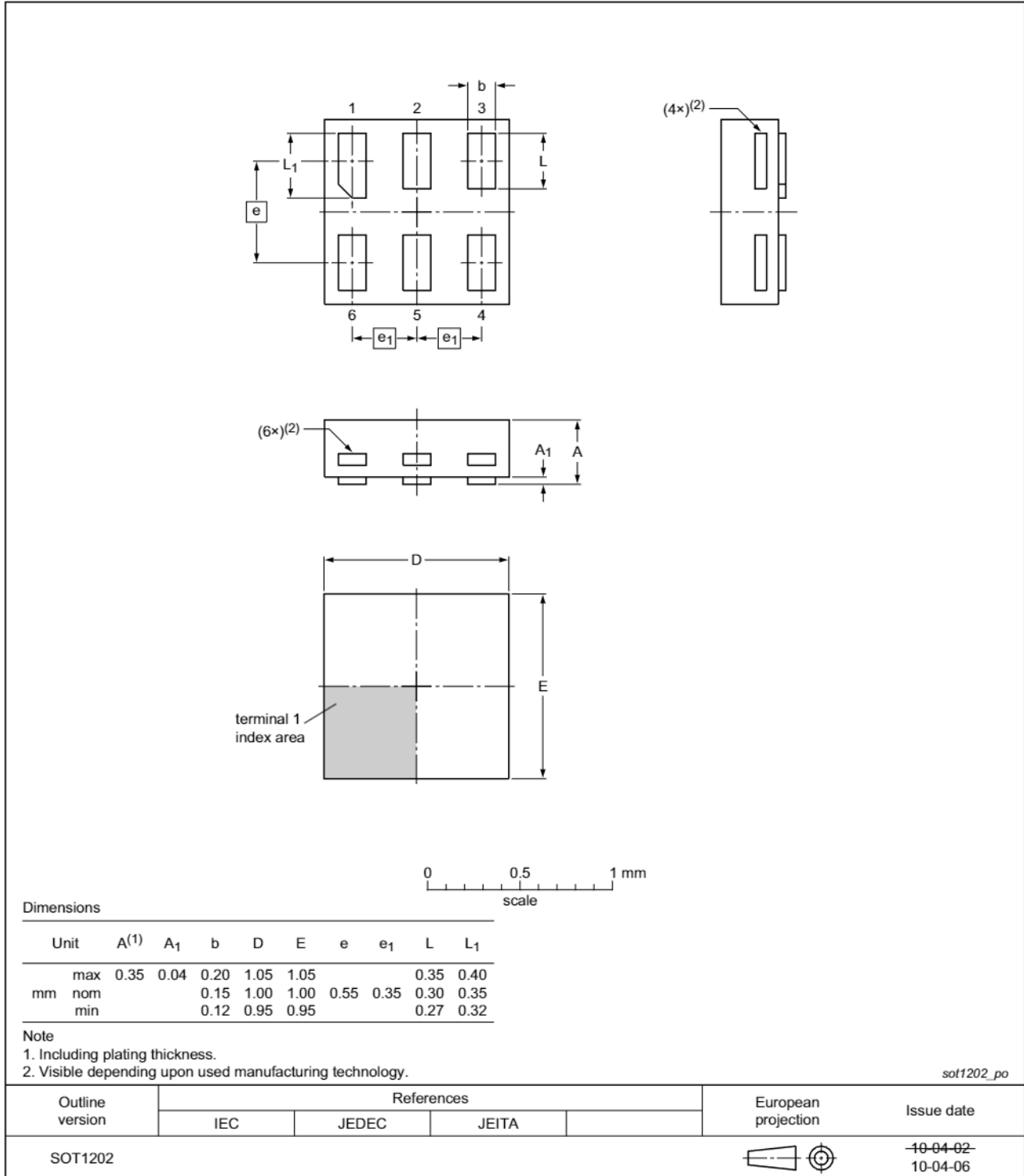
Fig 22. Package outline SOT1202 (XSON6)
