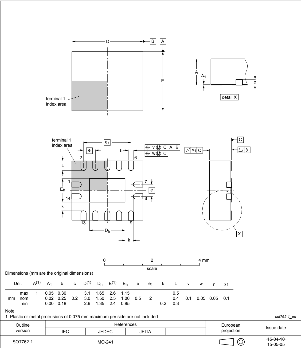
Figure 19. Package outline SOT762-1 (DHVQFN14)
