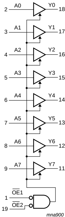
Fig 2. Functional diagram
