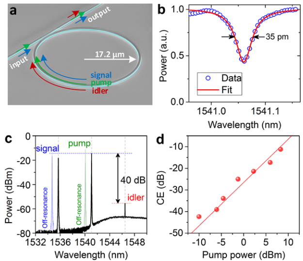
Figure 5. FWM characterization of the AlGaAsOI microresonator. a) SEM picture of a fabricated AlGaAsOI microresonator with a radius of 17.2\ \mu\text{m} . b) Measured normalized transmission spectrum of an over-coupled AlGaAsOI microresonator at 1540\ \text{nm} . The resonance linewidth is \approx 35\ \text{pm} which corresponds to a Q factor of 44000. c) Measured output spectra of the microresonator with the pump and signal waves off-resonance (colored curves) and on-resonance (black curve). The light gray dashed lines show the resonance wavelengths of the microresonator. d) Measured FWM conversion efficiency (CE) for the microresonator as a function of the pump power in the bus waveguide.
