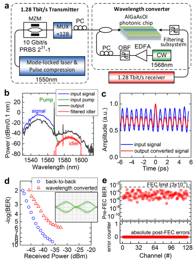
Figure 4. Wavelength conversion experiment. a) Experimental setup for all-optical wavelength conversion of a 1.28 Tbit s -1 DPSK data signal. b) Spectra at the input, output of the AlGaAsOI nano-waveguide and the converted signal after filtering. c) Autocorrelation trace of the input signal and the output converted signal. d) BER measurements for the 1.28 Tbit s -1 back-to-back and the wavelength-converted signal. Inset: eye diagram of a 10 Gbit s -1 demultiplexed channel from the 1.28 Tbit s -1 converted signal. e) BER for all the 128 OTDM tributaries of the 1.28 Tbit s -1 converted signal.
