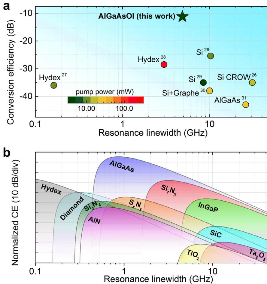
Figure 6. CW-FWM performance comparison for microresonators. a) Summary of experimentally achieved conversion efficiency versus the resonance linewidth for microresonators in different material platforms. b) Estimated FWM performance for microresonators in emerging two-photon absorption (TPA)-free material platforms. The FSRs are assumed the same in the theoretical analysis.
