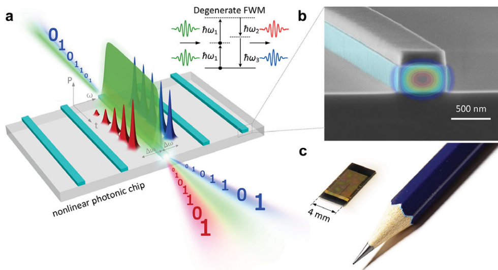
Figure 1. Nonlinear photonic chip for optical signal processing (OSP). a) Schematic illustration of an example OSP: all-optical wavelength conversion of data signals based on degenerate four-wave mixing (FWM) in a nonlinear waveguide on a photonic chip. b) Scanning electron microscopy (SEM) picture of an AlGaAs-on-insulator (AlGaAsOI) nano-waveguide (denoted by artificial blue color) fabricated by electron-beam lithography and inductive-coupled plasma dry etching process. The top left-over layer is the electron-beam resist which is used as an etching mask for patterning. The simulated field distribution for the fundamental TE mode is superimposed on the image showing strong light confinement. c) Photograph of a pencil and a fabricated 4-mm-wide AlGaAsOI photonic chip accommodating hundreds of waveguide-based devices.
