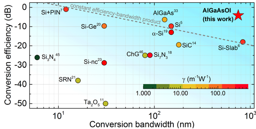
Figure 3. CW-FWM performance comparison. Summary of experimentally achieved conversion efficiency and bandwidth for FWM at telecom wavelengths in straight waveguides in different material platforms. The gray dashed line is used as a guide for the eyes showing a constant efficiency-bandwidth product.
