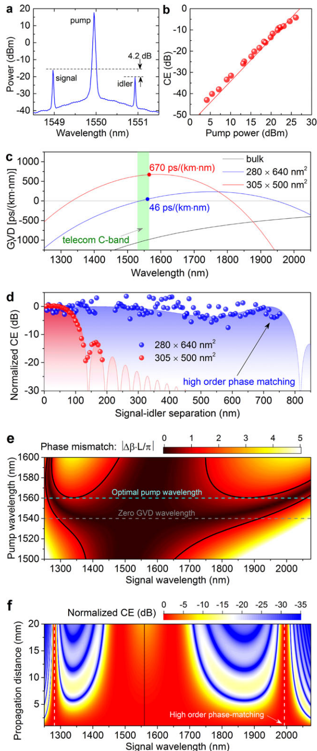
Figure 2. FWM characterization of AlGaAsOI nano-waveguides. a) Measured optical output spectrum of a 3-mm-long AlGaAsOI nano-waveguide (cross-sectional dimension: 280 \times 640 \text{ nm}^2 ) when a pump wave (1550 nm, 400 mW) and a signal wave (1549 nm, 100 \mu\text{W} ) are coupled into the device under continuous-wave (CW) operation. b) Measured output FWM conversion efficiency (CE) as a function of pump power for the device. The pump wavelength is set in the telecom C-band. c) Cal-
