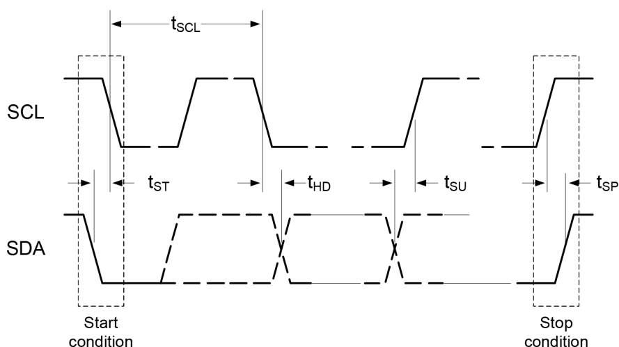
Figure 1: I 2 C Compatible Serial Bus Timing
