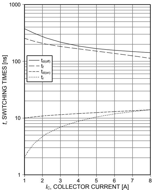
Figure 7. Typical switching times as a function of collector current (inductive load, T vj =175°C, V CE =400V, V GE =15/0V, r G =43Ω, Dynamic test circuit in Figure E)
