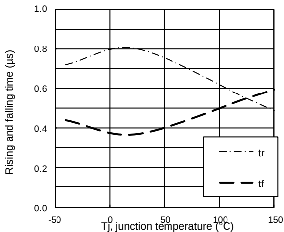
Figure 7 – tr / tf (μs) Vs Tj (°C)
