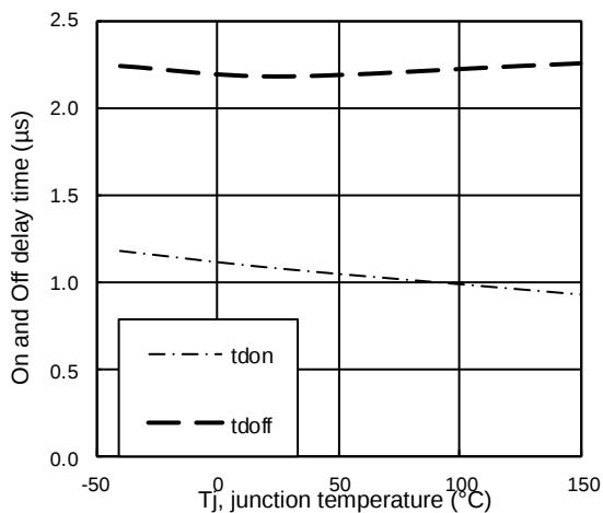
Figure 8 – tdon / tdoff (μs) Vs Tj (°C)
