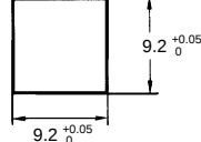
Panel Cutout of B32-12□0
