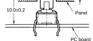
Panel Cutout of B32-13□0
