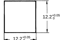
Panel Cutout of B32-13□0
