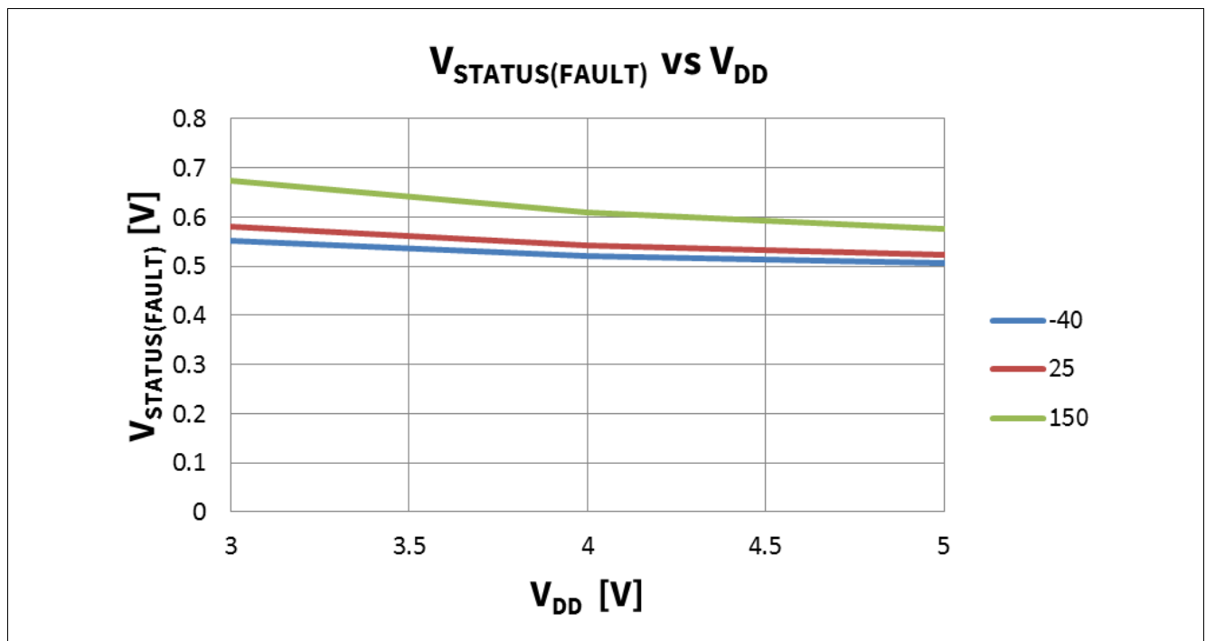
Figure 44 V_{\text{STATUS}} in fault mode vs. V_{\text{DD}} = 3\text{V} \dots 5\text{V} @ T_{\text{J}} = -40, 25, 150^\circ\text{C} ; V_{\text{IN}} = V_{\text{ENABLE}} = 5\text{V} ; V_{\text{BAT}} = 13.5\text{V} ;
