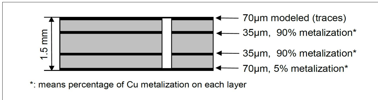
Figure 4 Cross-section JEDEC2s2p
