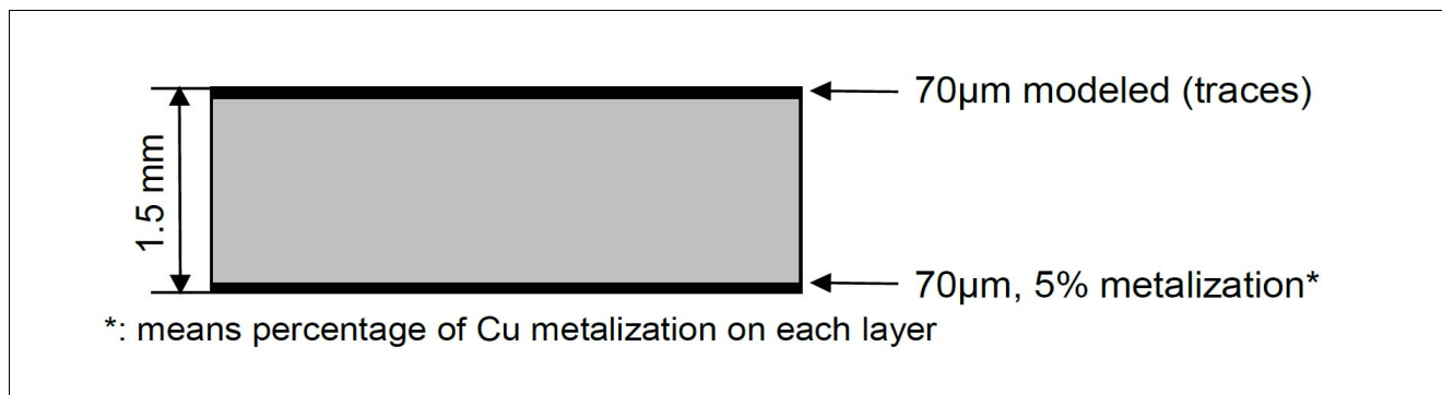
Figure 5 Cross-section JEDEC1s0p
