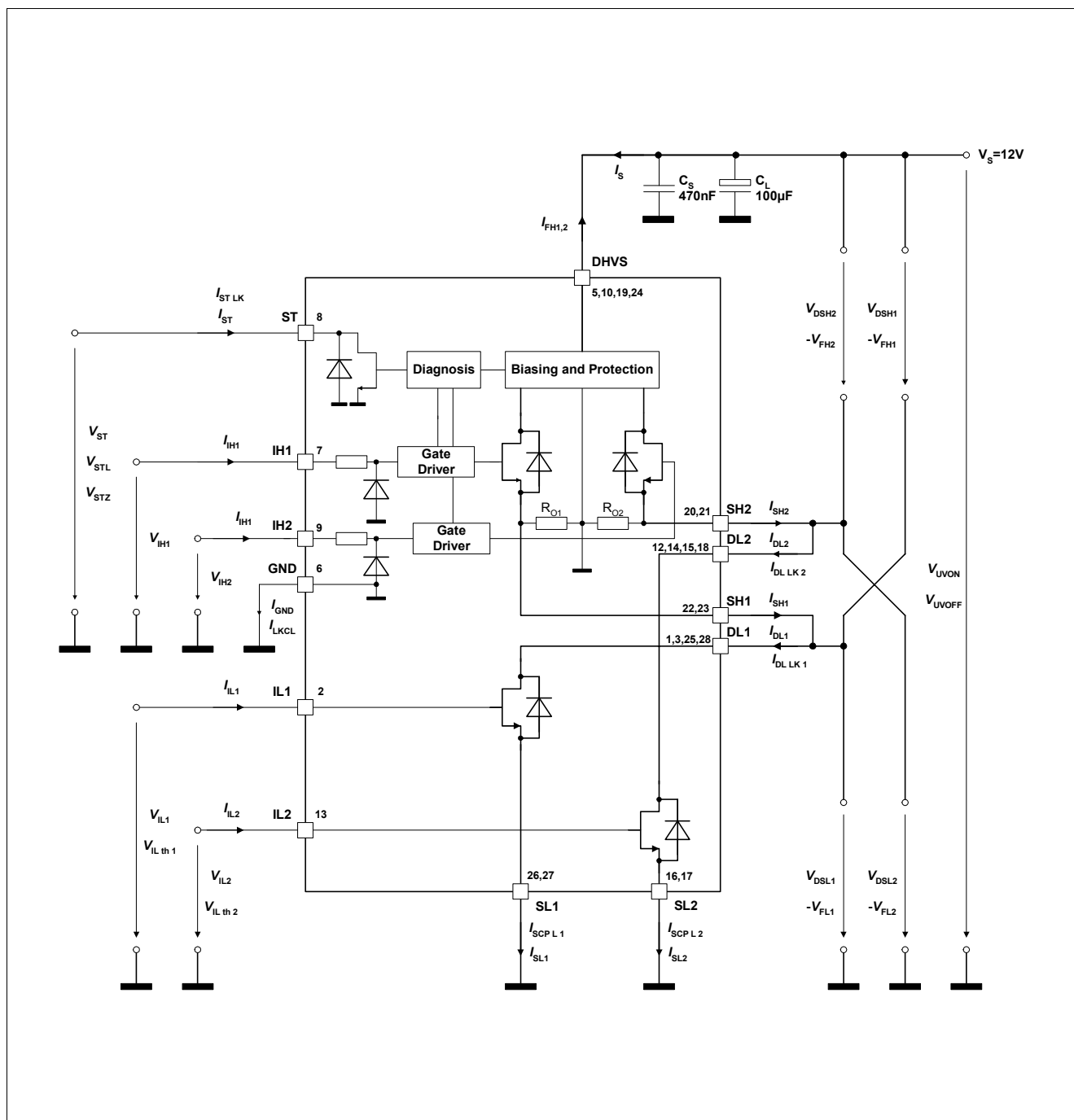
Figure 2 Terms BTM7710G
