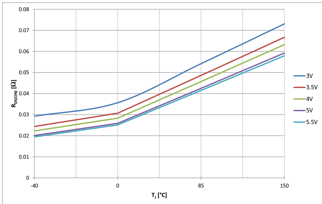
Figure 18 Typical R_{DS(ON)} vs. T_J @ V_{IN} = 3 \dots 5.5 \text{ V} , I_L = I_{L(NOM)}
