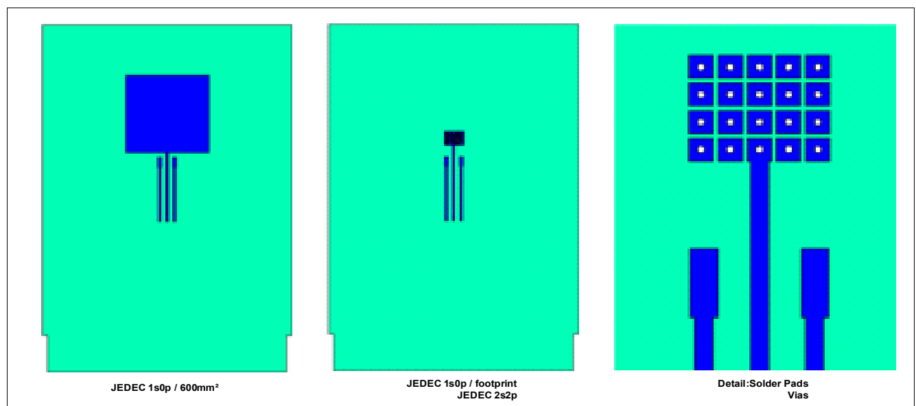
Figure 6 PCB layout
