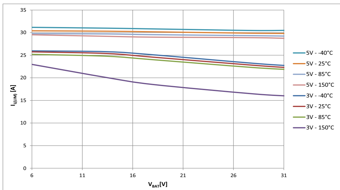
Figure 38 Typical I_{L(LIM)} vs. V_{BAT} @ T_J = -40 \dots 150^\circ\text{C} , V_{IN} = 3 V and 5 V
