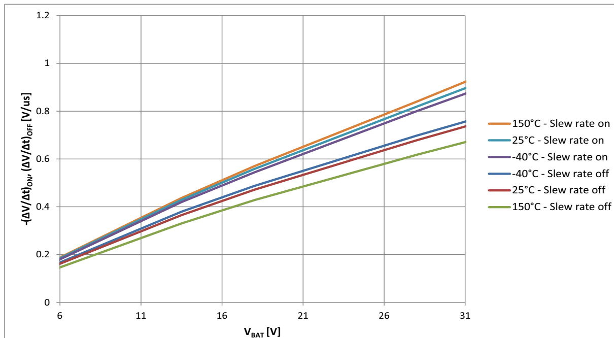
Figure 30 Typical -(\Delta V/\Delta t)_{ON} , (\Delta V/\Delta t)_{OFF} vs. V_{BAT} @ V_{IN} = 5V ; T_J = -40 \dots 150^\circ C
