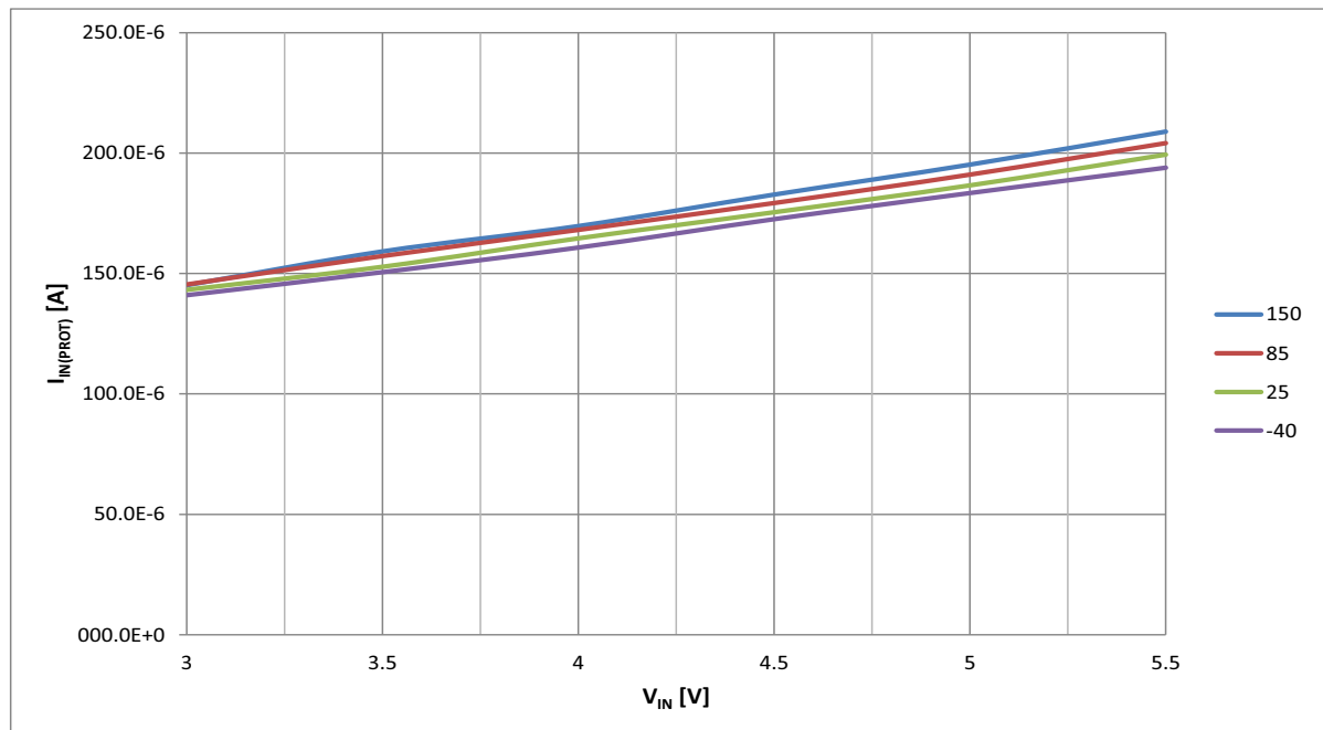
Figure 41 Typical I_{IN(Prot)} vs. V_{IN} @ T_J = -40 \dots 150^\circ\text{C} , I_L = I_{L(NOM)}
