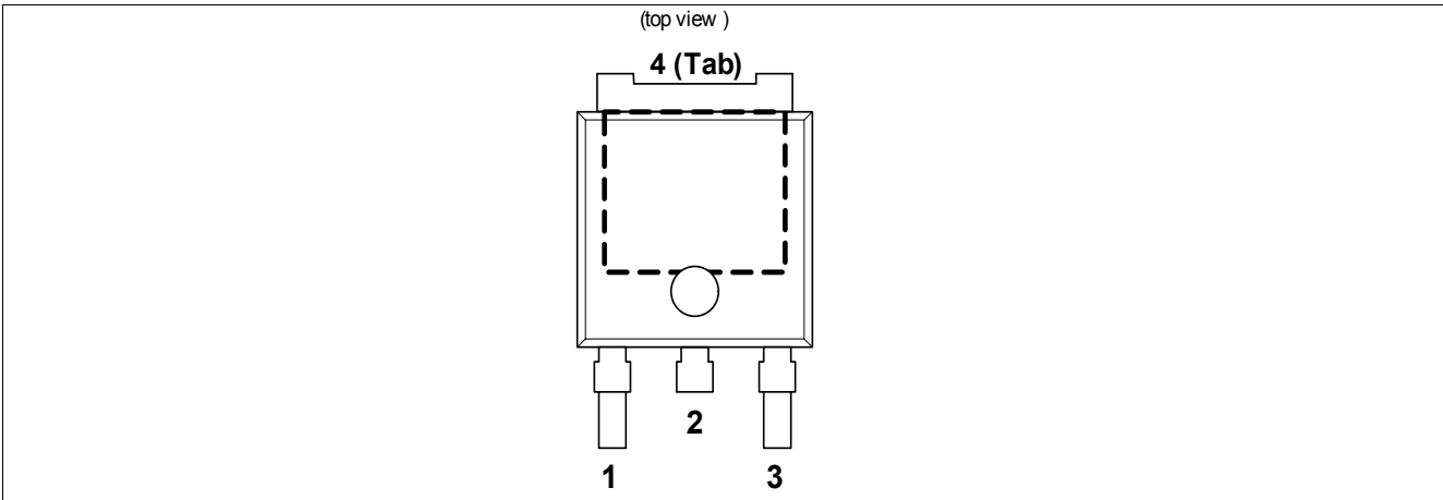
Figure 2 Pin Configuration. PG-T0252-3
