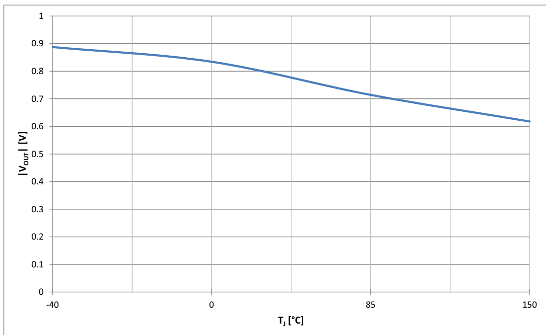
Figure 19 Typical Reverse Diode |V_{OUT}| vs. T_J @ I_L = I_{L(NOM)}
