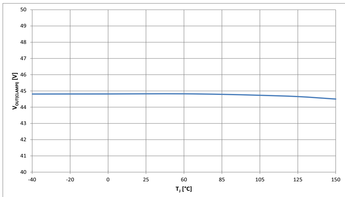
Figure 37 Typical V_{OUT(CLAMP)} vs. T_J @ I_L = 14 mA
