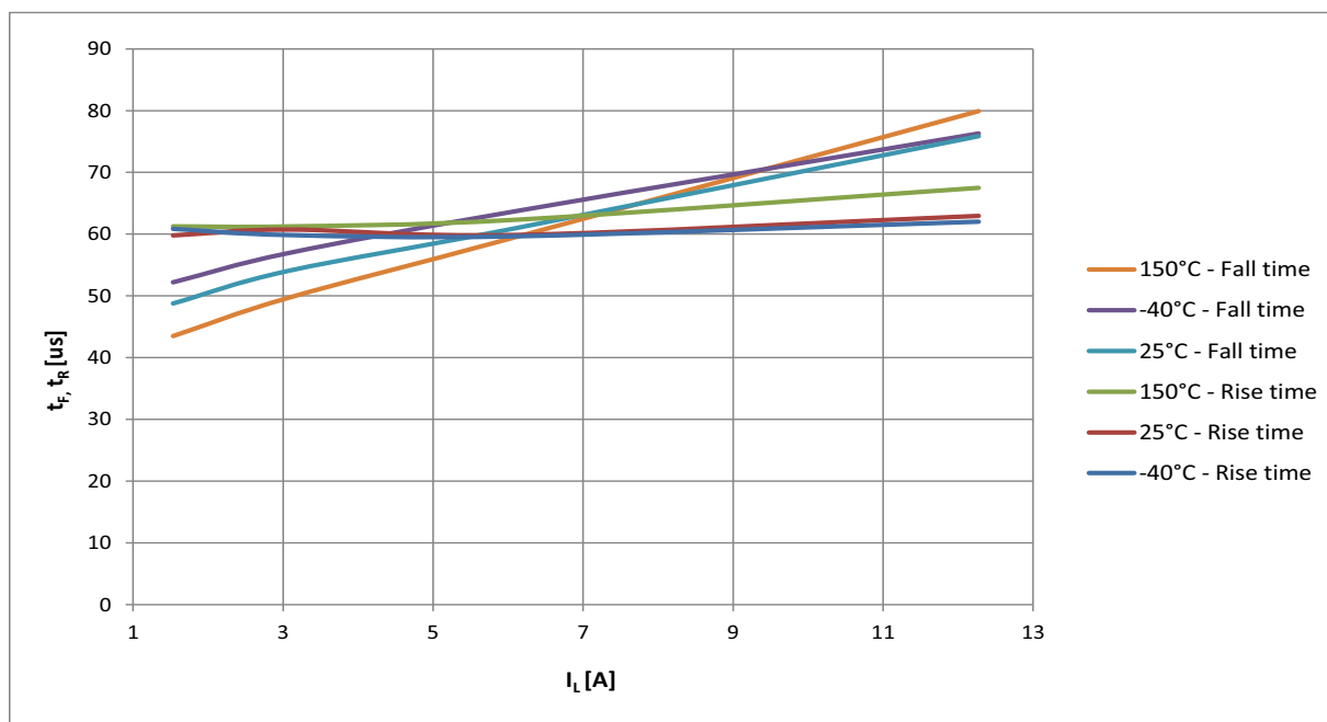
Figure 31 Typical t_F , t_R vs. I_L @ V_{IN} = 5V ; T_J = -40 \dots 150^\circ C
