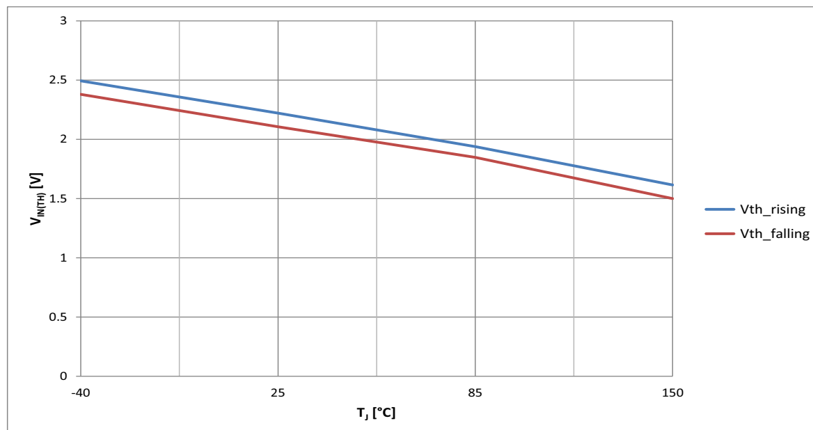
Figure 39 Typical V_{IN(TH)} vs. T_J @ I_L = 1.4 mA
