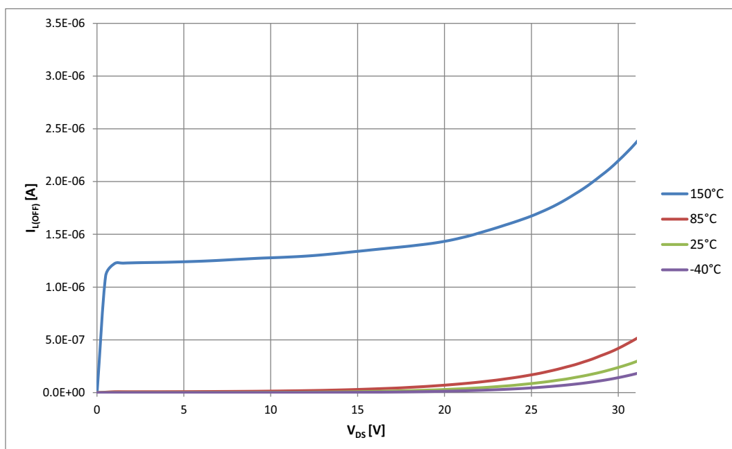
Figure 20 Typical I_{L(OFF)} vs. V_{DS} @ T_J = -40 \dots 150^\circ\text{C} , V_{IN} = 0\text{ V}
