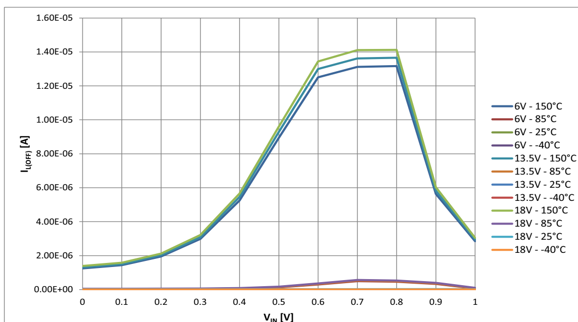
Figure 21 Typical I_{L(OFF)} vs. V_{IN} @ T_J = -40 \dots 150^\circ\text{C} , V_{BAT} = 6 \dots 18\text{ V}
