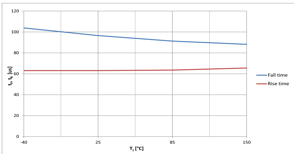
Figure 34 Typical t_F , t_R vs. T_J @ V_{IN} = 5\text{ V}
