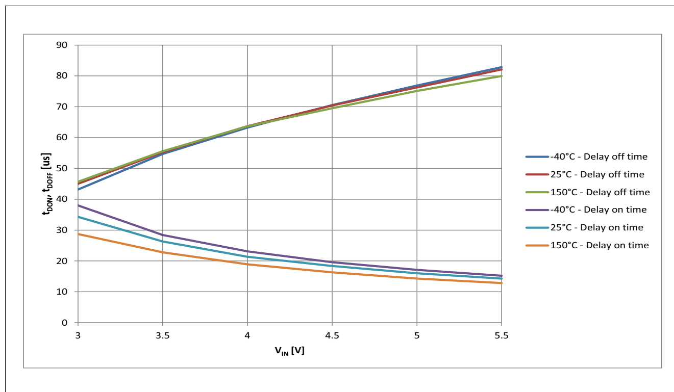
Figure 26 Typical t_{DON} , t_{DOFF} vs. V_{IN} @ T_J = -40 \dots 150^\circ C
