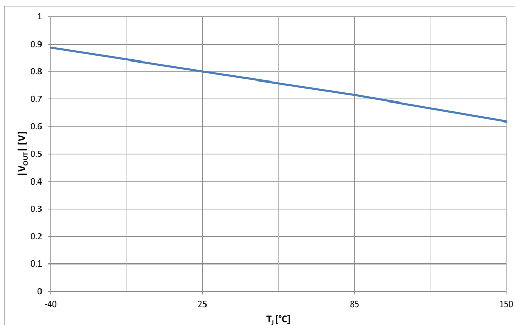
Figure 19 Typical Reverse Diode |V_{OUT}| vs. T_J @ I_L = I_{L(NOM)}
