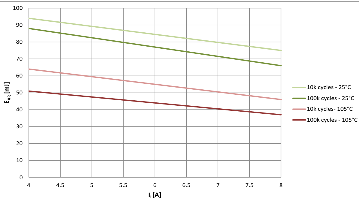
Figure 23 Typical E_{AR} vs. I_L @ T_J = 25 and 105^\circ\text{C} , V_{BAT} = 13.5\text{V}
