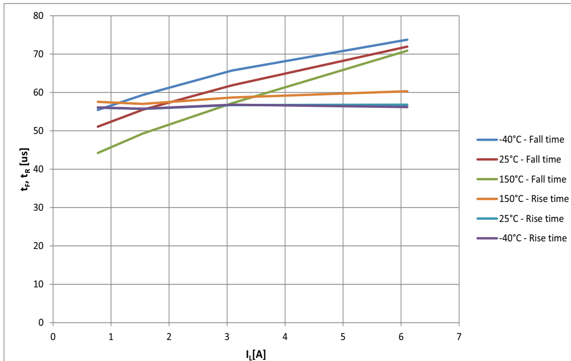
Figure 31 Typical t_F , t_R vs. I_L @ V_{IN} = 5V ; T_J = -40 \dots 150^\circ C
