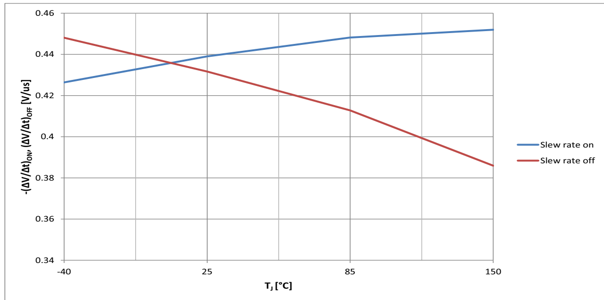
Figure 36 Typical -(\Delta V/\Delta t)_{ON} , (\Delta V/\Delta t)_{OFF} vs. T_J @ V_{IN} = 5\text{ V}
