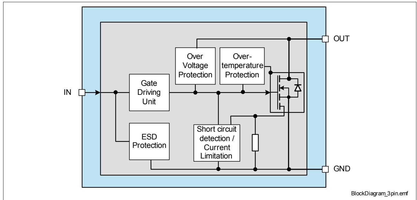
Figure 1 Block Diagram
