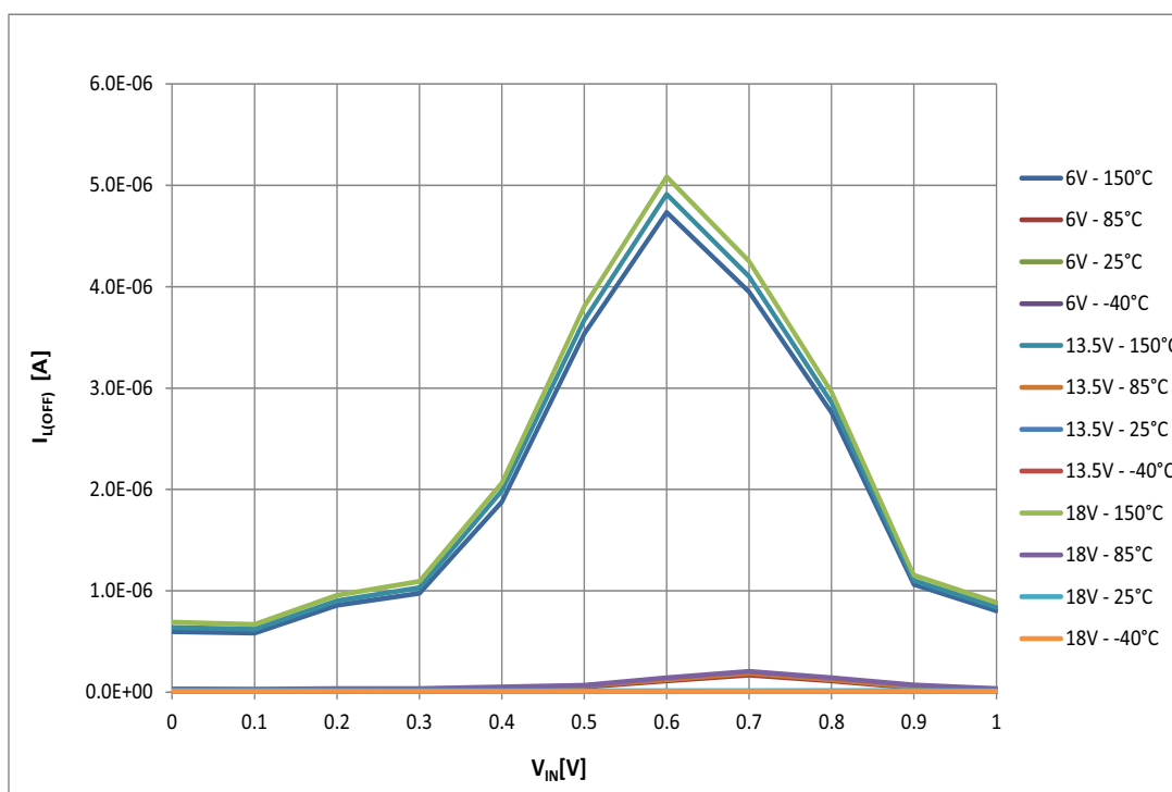
Figure 21 Typical I_{L(OFF)} vs. V_{IN} @ T_J = -40 \dots 150^\circ\text{C} , V_{BAT} = 6 \dots 18\text{ V}
