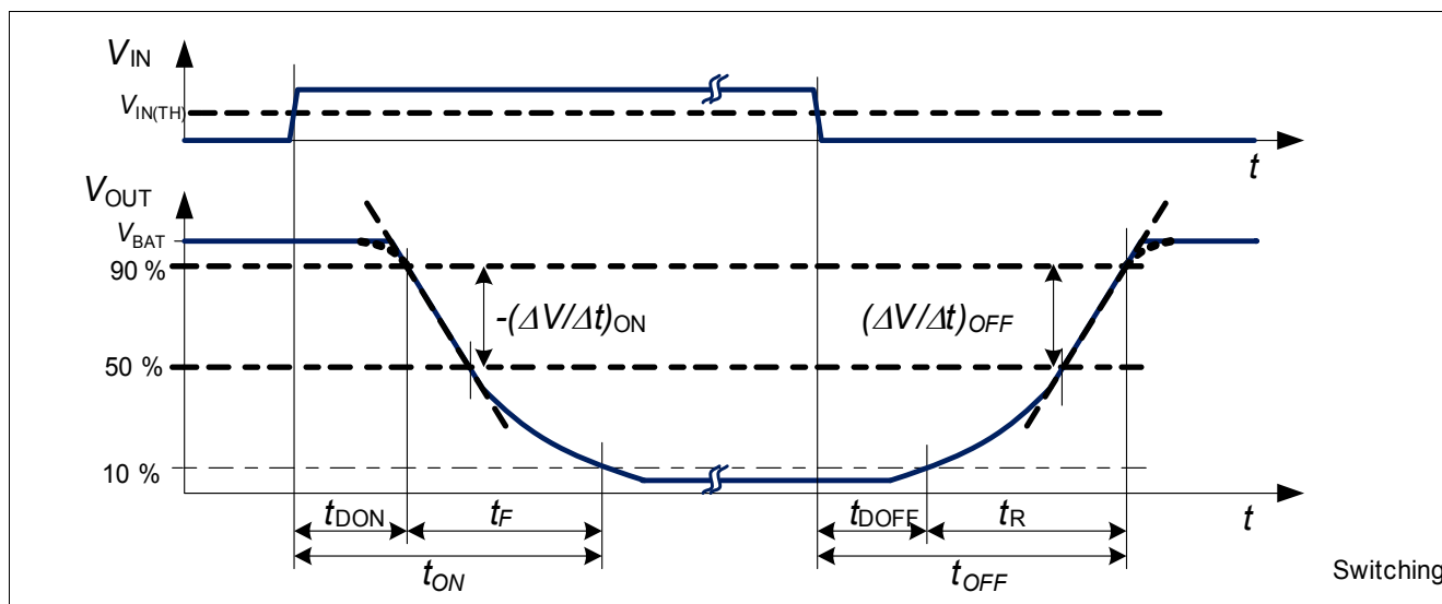
Figure 10 Definition of Power Output Timing for Resistive Load
