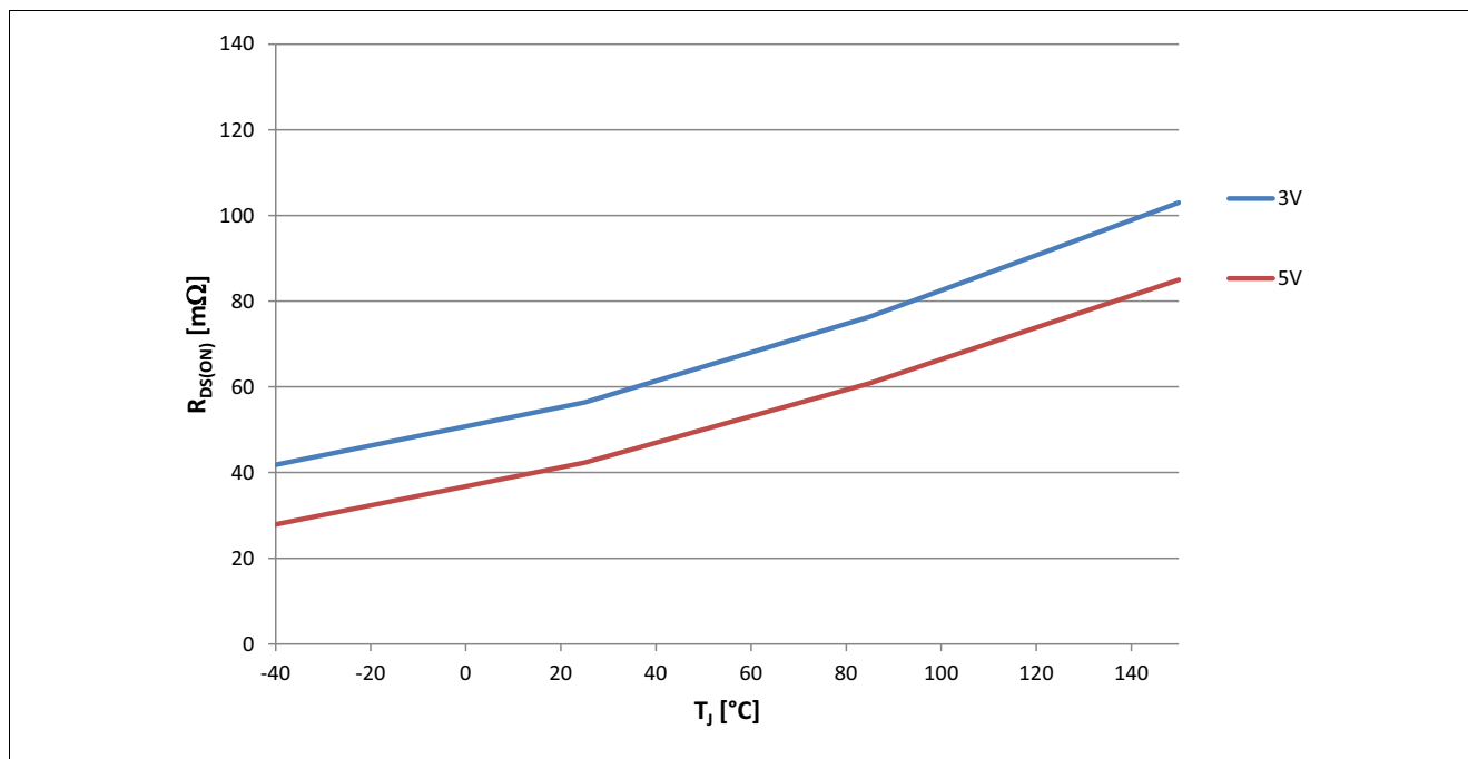
Figure 9 Typical On-State Resistance, R_{DS(ON)} = f(T_J) , V_{IN} = 3V ; V_{IN} = 5V
