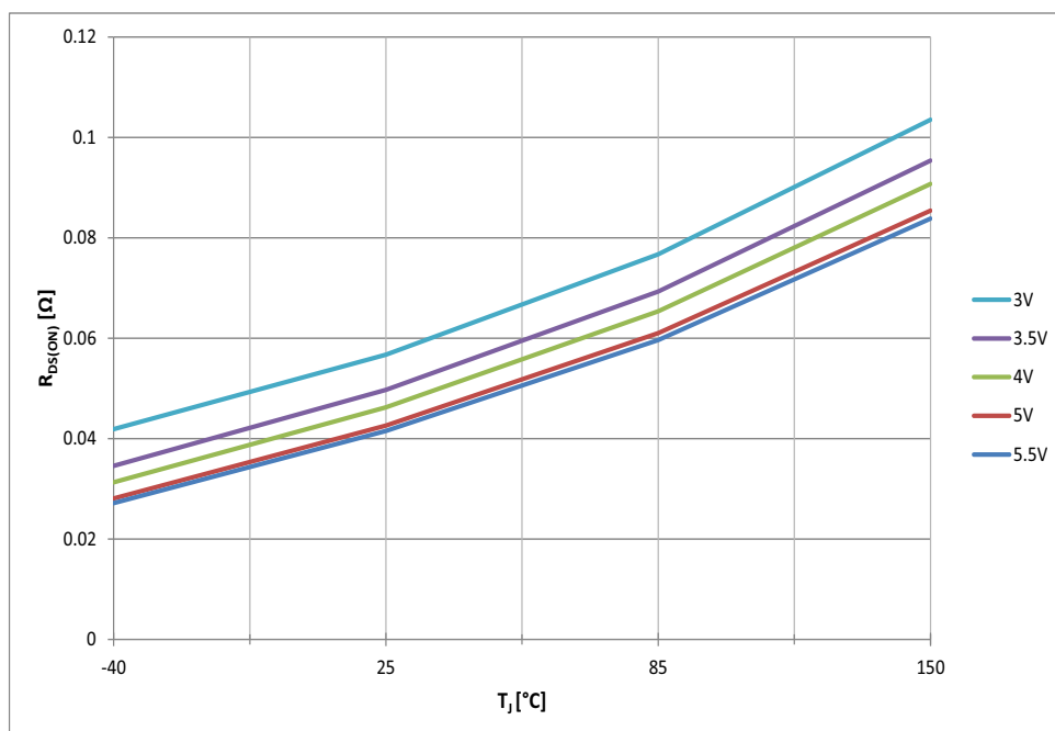
Figure 18 Typical R_{DS(ON)} vs. T_J @ V_{IN} = 3 \dots 5.5 \text{ V} , I_L = I_{L(NOM)}
