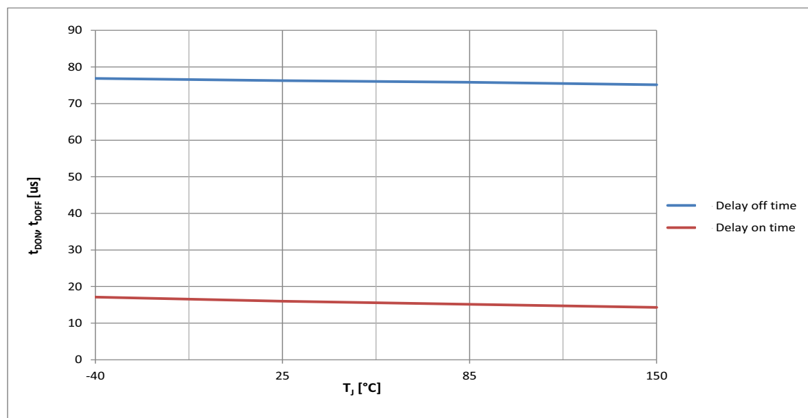
Figure 35 Typical t_{DON} , t_{DOFF} vs. T_J @ V_{IN} = 5\text{ V}
