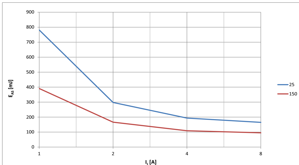
Figure 22 Typical destruction point. E_{AS} vs. I_L @ T_J = 25 and 150^\circ\text{C} , V_{BAT} = 13.5\text{V}
