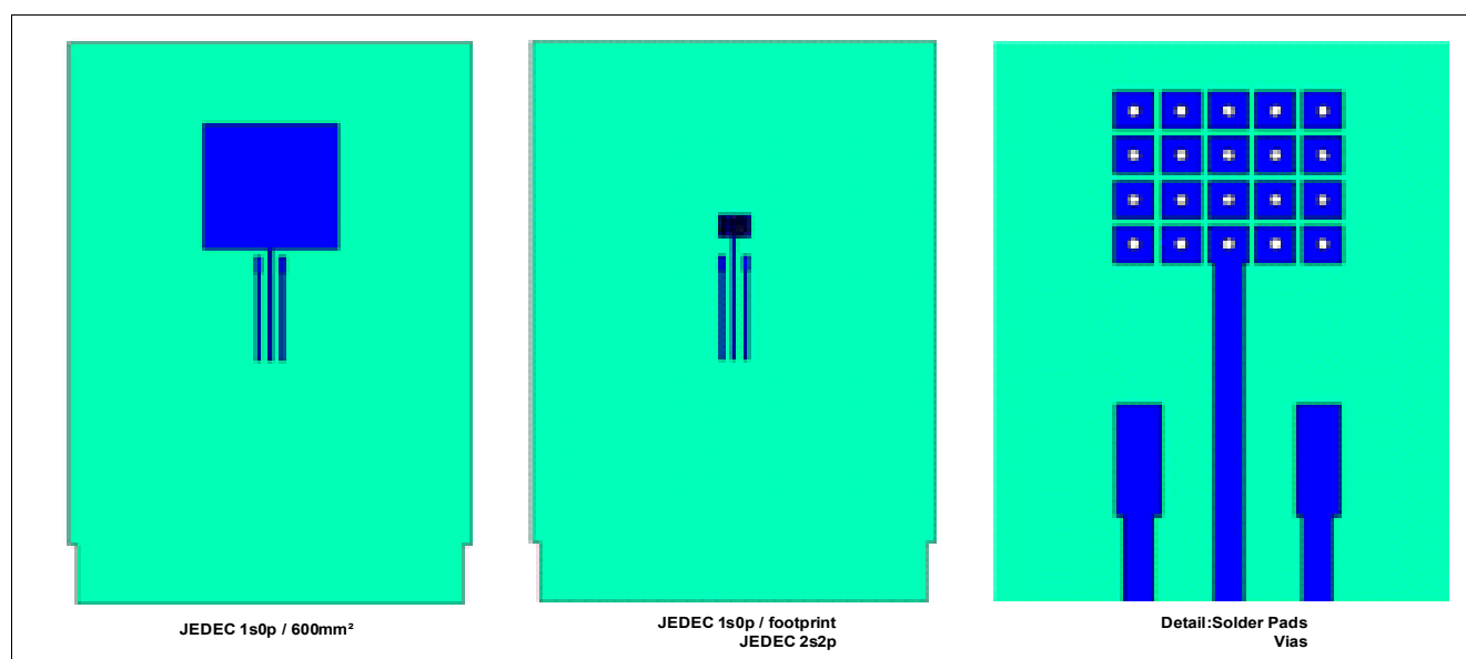
Figure 6 PCB layout
