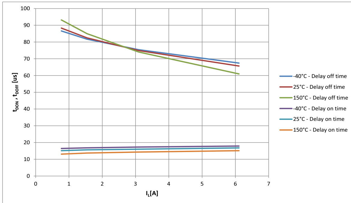
Figure 32 Typical t_{\text{DON}} , t_{\text{DOFF}} vs. I_L @ V_{\text{IN}} = 5\text{V} ; T_J = -40 \dots 150^\circ\text{C}
