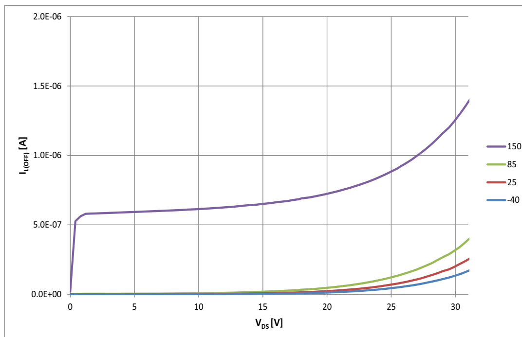
Figure 20 Typical I_{L(OFF)} vs. V_{DS} @ T_J = -40 \dots 150^\circ\text{C} , V_{IN} = 0\text{ V}
