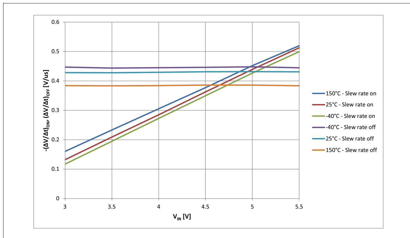
Figure 27 Typical -(\Delta V/\Delta t)_{ON} , (\Delta V/\Delta t)_{OFF} vs. V_{IN} @ T_J = -40 \dots 150^\circ C
