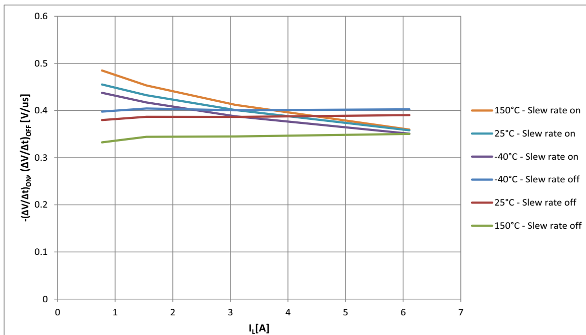
Figure 33 Typical -(\Delta V/\Delta t)_{\text{ON}} , (\Delta V/\Delta t)_{\text{OFF}} vs. I_L @ V_{\text{IN}} = 5\text{V} ; T_J = -40 \dots 150^\circ\text{C}
