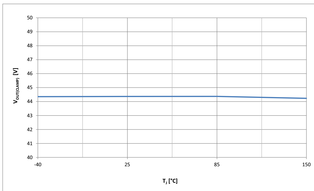
Figure 37 Typical V_{OUT(CLAMP)} vs. T_J @ I_L = 10 mA
