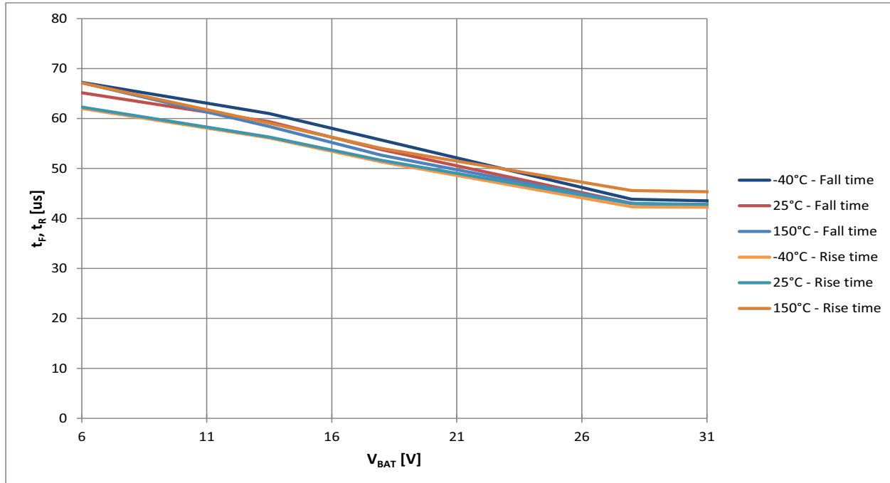
Figure 28 Typical t_F , t_R vs. V_{BAT} @ V_{IN} = 5V ; T_J = -40 \dots 150^\circ C
