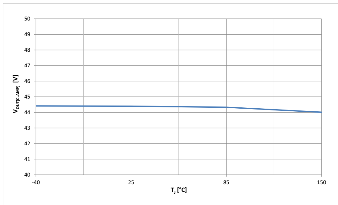
Figure 37 Typical V_{OUT(CLAMP)} vs. T_J @ I_L = 6\text{ mA}
