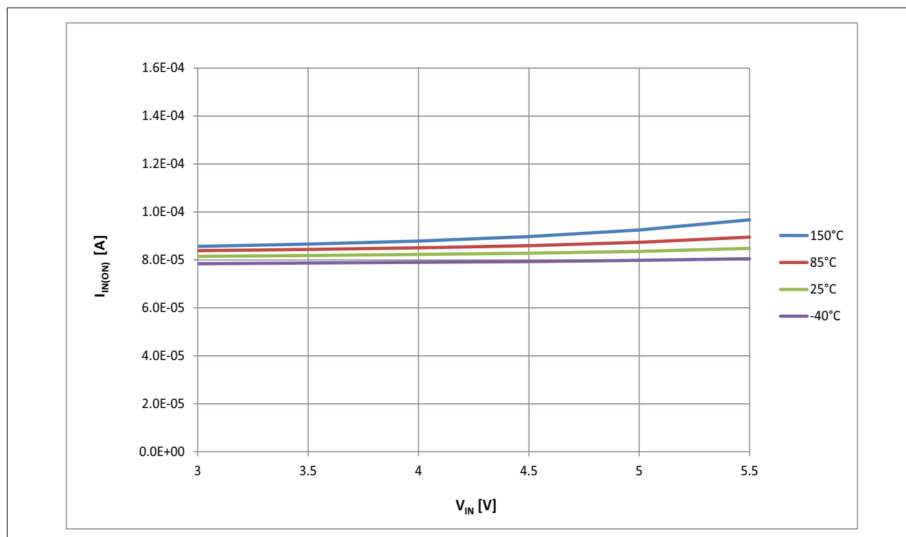
Figure 40 Typical I_{IN(ON)} vs. V_{IN} @ T_J = -40 \dots 150^\circ\text{C} , I_L = I_{L(NOM)}
