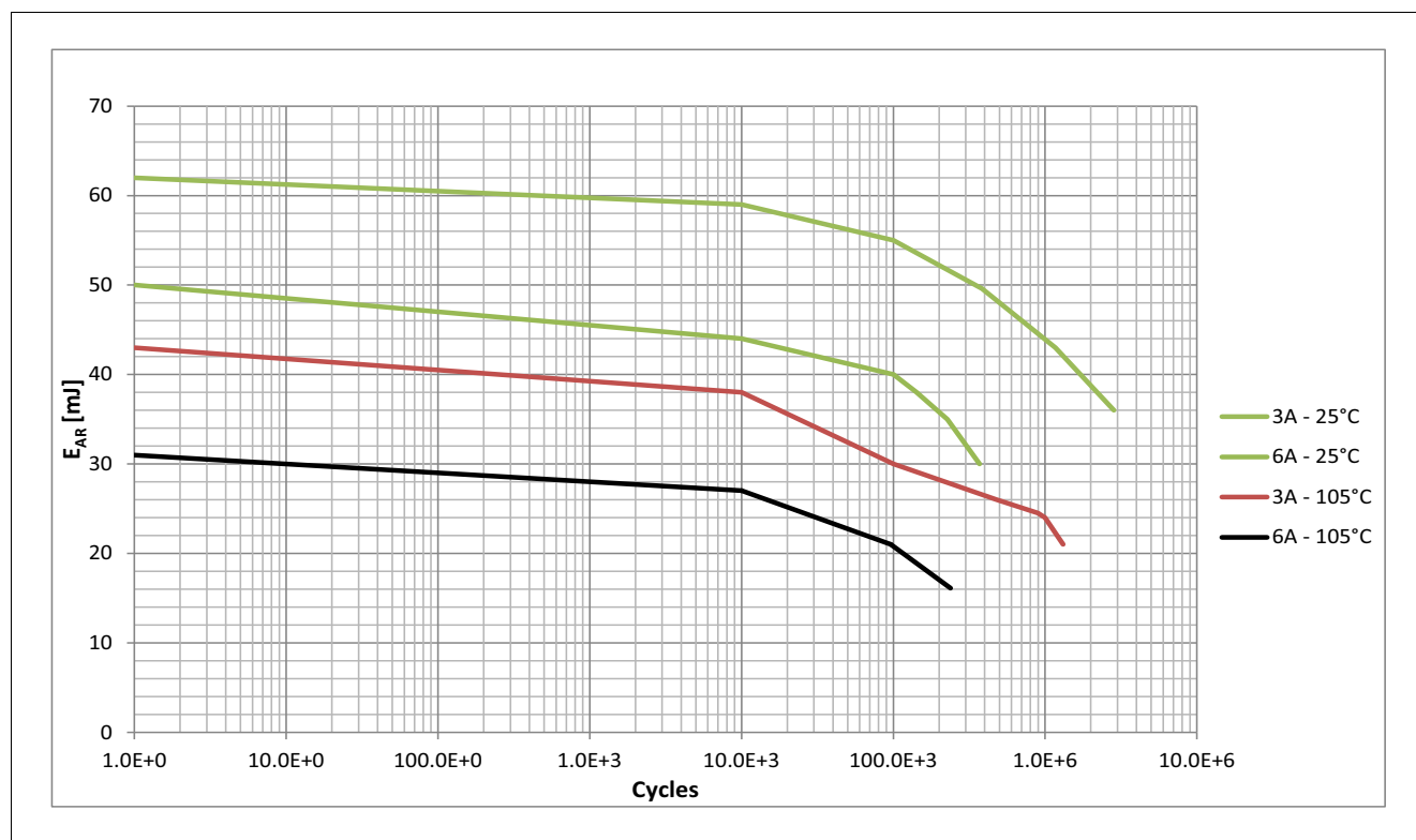
Figure 24 Typical E_{AR} vs. Cycles @ T_J = 25 and 105^\circ\text{C} , V_{BAT} = 13.5\text{V}
