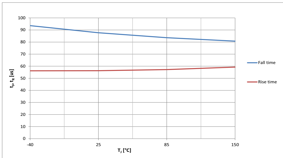
Figure 34 Typical t_F , t_R vs. T_J @ V_{IN} = 5\text{ V}
