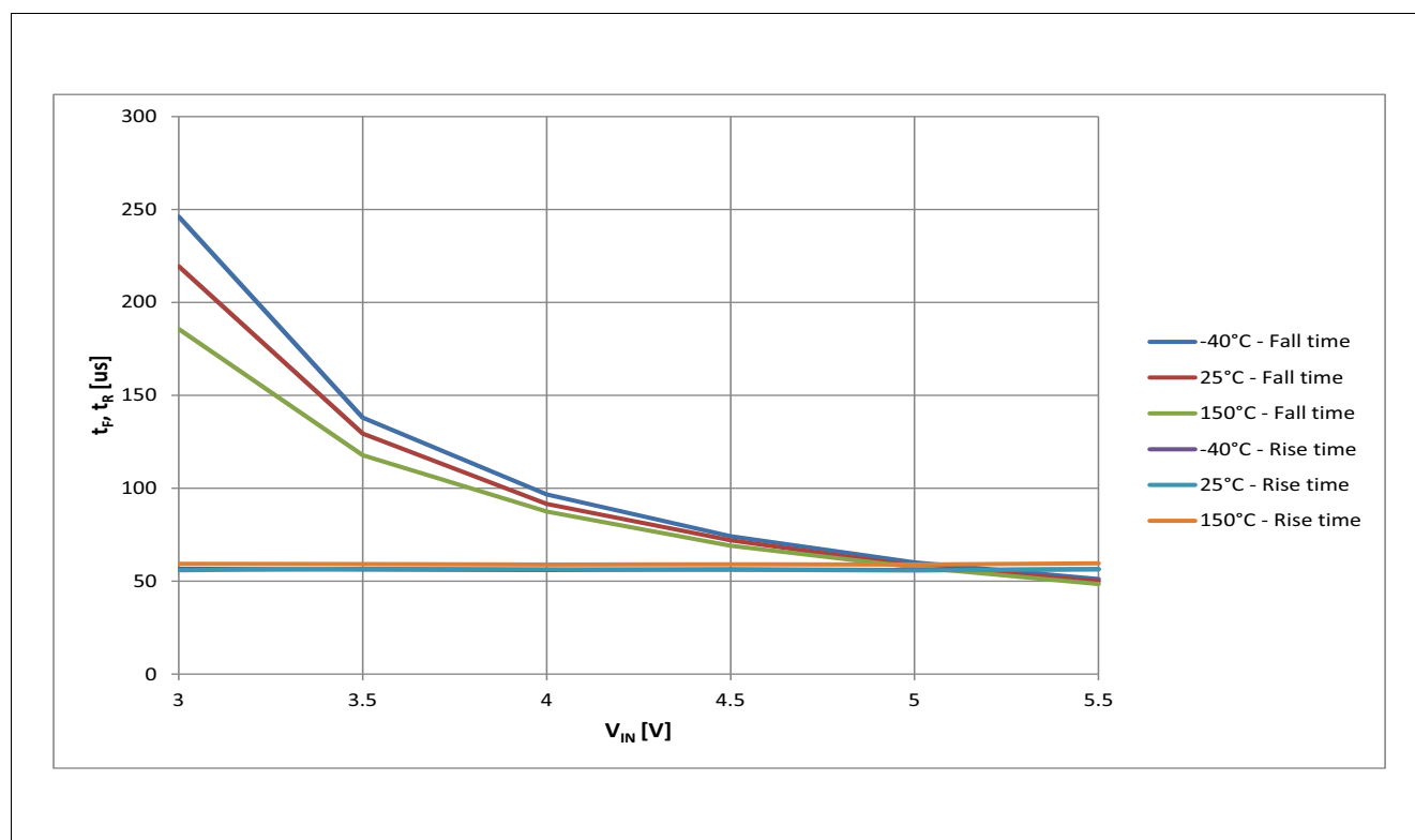
Figure 25 Typical t_F , t_R vs. V_{IN} @ T_J = -40 \dots 150^\circ\text{C}
