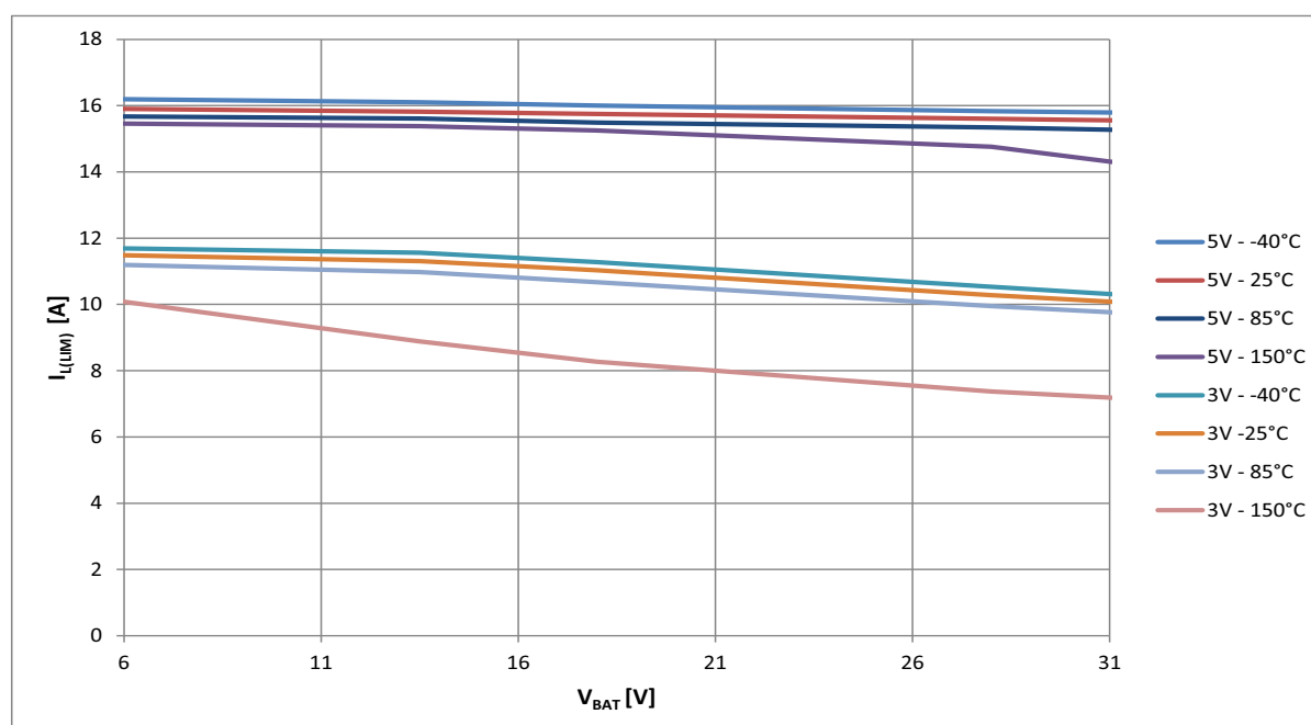
Figure 38 Typical I_{L(LIM)} vs. V_{BAT} @ T_J = -40 \dots 150^\circ\text{C} , V_{IN} = 3\text{ V and } 5\text{ V}
