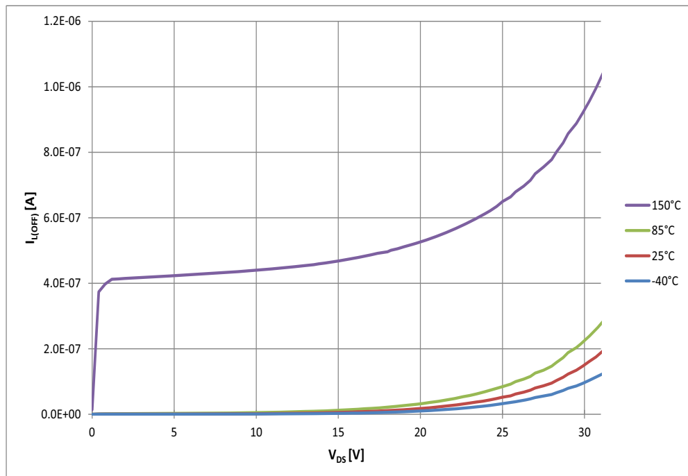
Figure 20 Typical I_{L(OFF)} vs. V_{DS} @ T_J = -40 \dots 150^\circ\text{C} , V_{IN} = 0\text{ V}
