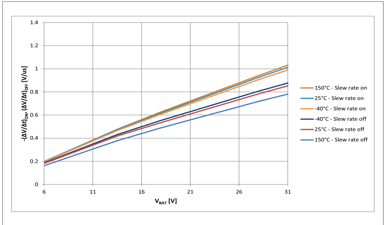
Figure 30 Typical -(\Delta V/\Delta t)_{ON} , (\Delta V/\Delta t)_{OFF} vs. V_{BAT} @ V_{IN} = 5V ; T_J = -40 \dots 150^\circ\text{C}
