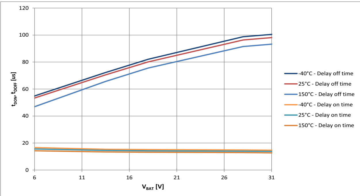
Figure 29 Typical t_{DON} , t_{DOFF} vs. V_{BAT} @ V_{IN} = 5V ; T_J = -40 \dots 150^\circ C
