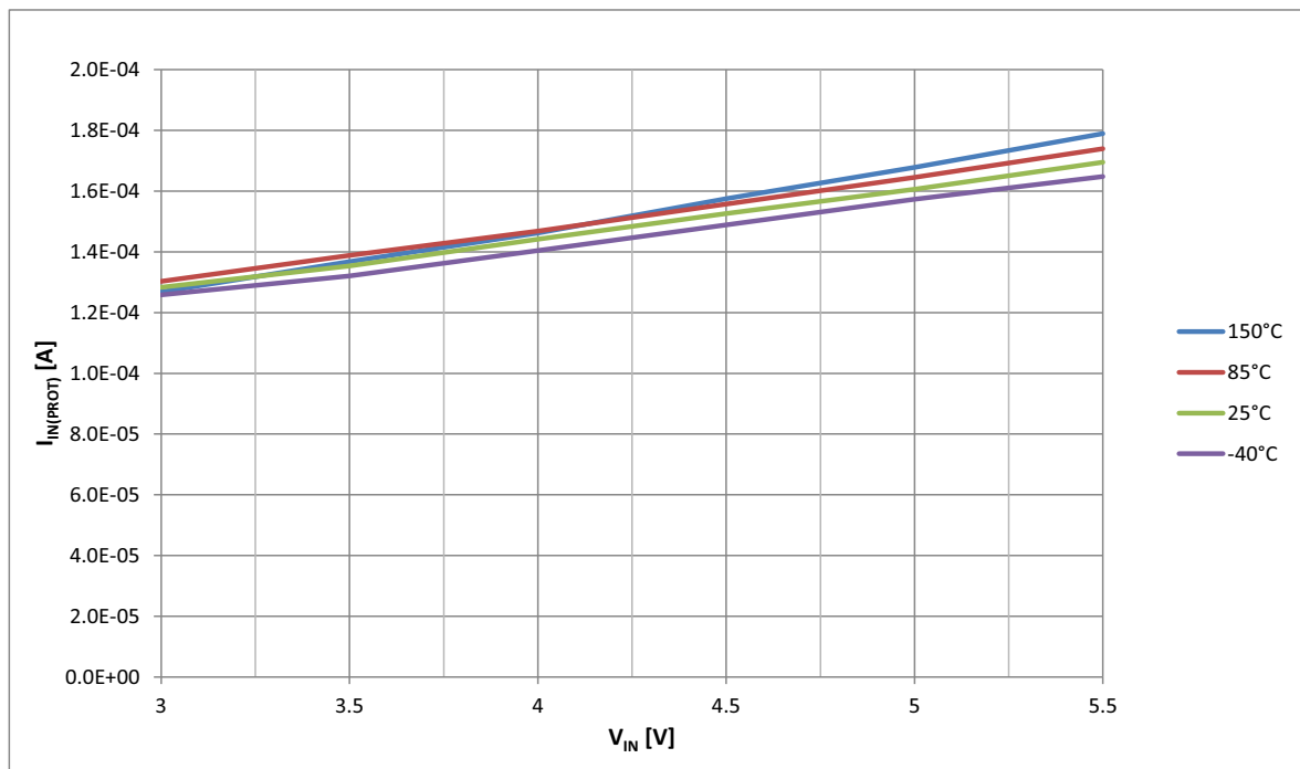
Figure 41 Typical I_{IN(PROT)} vs. V_{IN} @ T_J = -40 \dots 150^\circ\text{C} , I_L = I_{L(NOM)}
