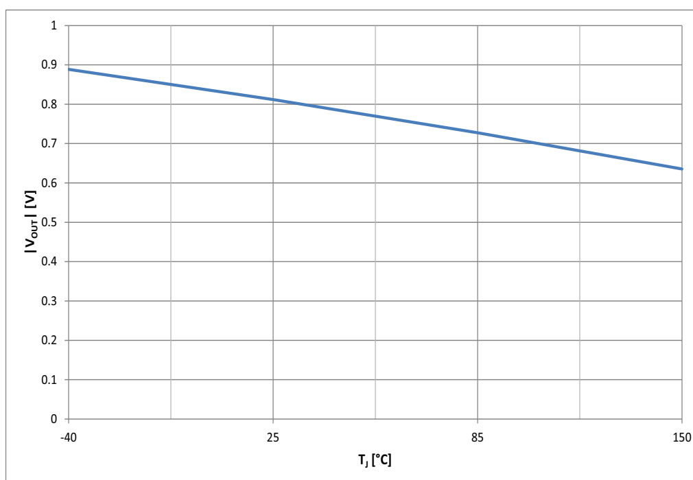
Figure 19 Typical Reverse Diode |V_{OUT}| vs. T_J @ I_L = I_{L(NOM)}
