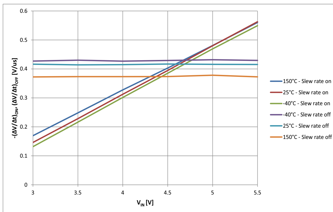
Figure 27 Typical -(\Delta V/\Delta t)_{ON} , (\Delta V/\Delta t)_{OFF} vs. V_{IN} @ T_J = -40 \dots 150^\circ\text{C}
