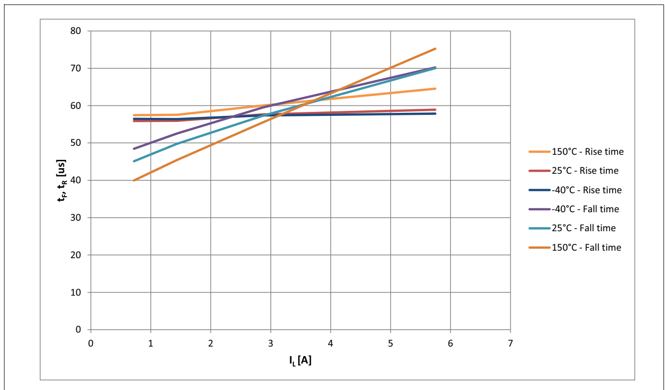
Figure 31 Typical t_F , t_R vs. I_L @ V_{IN} = 5V ; T_J = -40 \dots 150^\circ\text{C}
