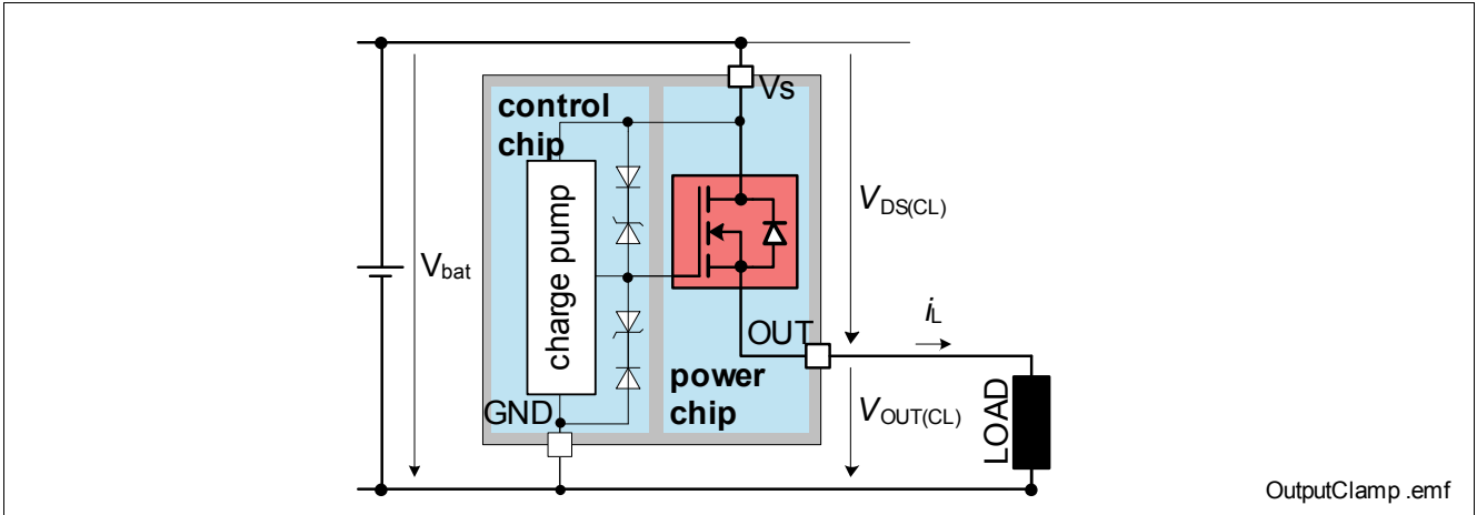
Figure 10 Output Clamp
