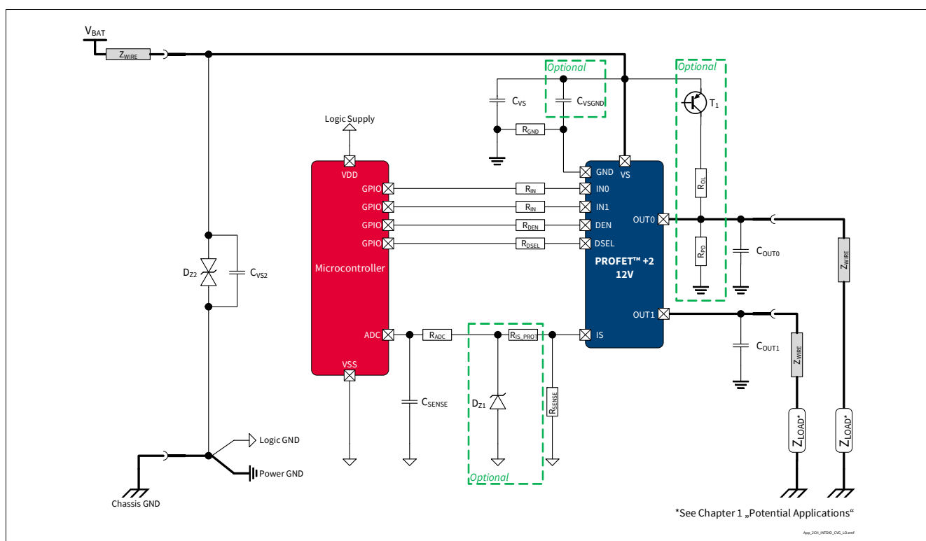
Figure 1 BTS7020-2EPA Application Diagram. Further information in Chapter 10
