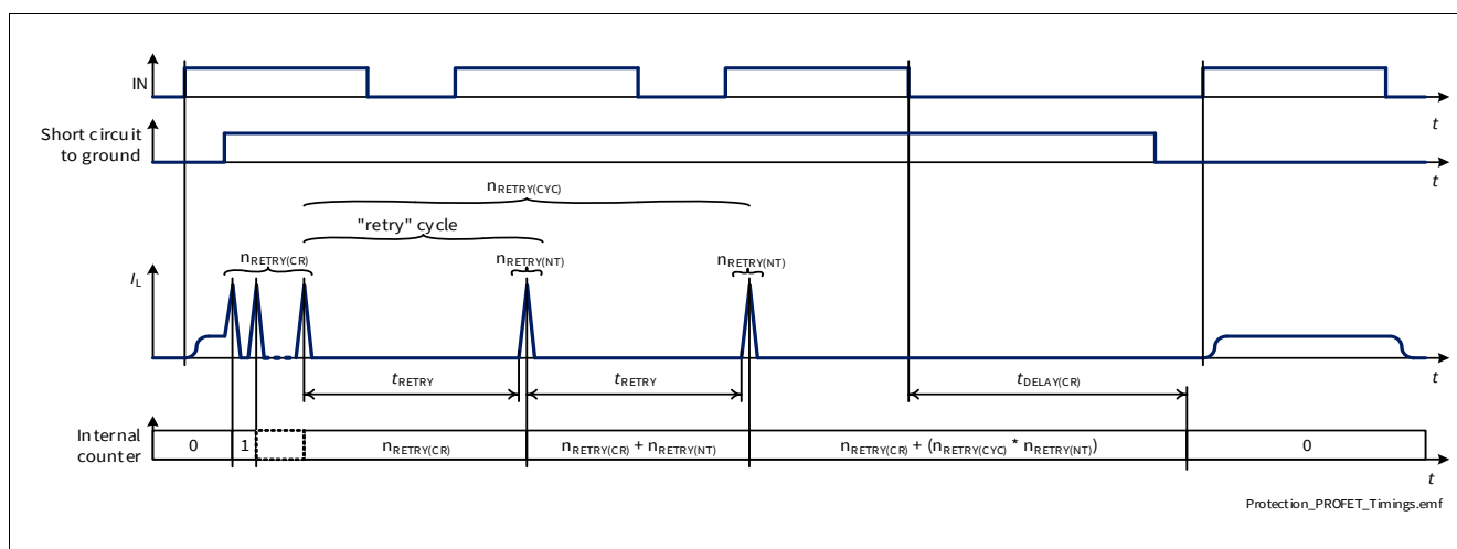
Figure 28 Retry Strategy Timing Diagram - Channel operated in PWM
