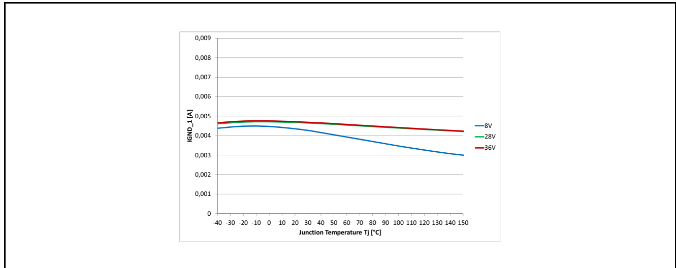
Figure 31 Current Consumption for Whole Device with Load. One Channel Active I_{\text{GND}_1} = f(T_j; V_s)
