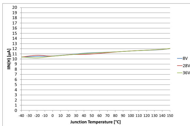
Figure 51 Input Current High Level I_{IN(H)} = f(T_J; V_S)
