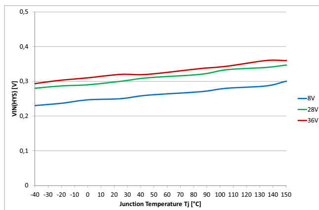
Figure 50 Input Voltage Hysteresis V_{IN(HYS)} = f(T_J; V_S)
