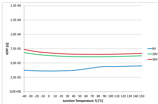
Figure 38 Turn OFF t_{OFF} = f(T_J; V_S) , R_L = 6 \Omega
