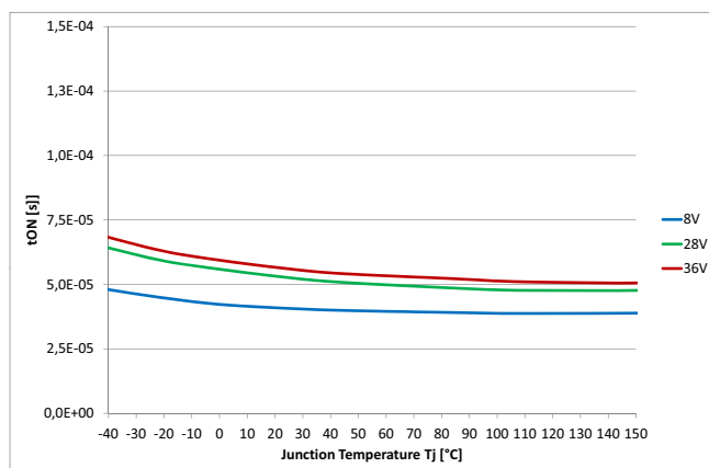
Figure 37 Turn ON t_{ON} = f(T_J; V_S) , R_L = 6 \Omega
