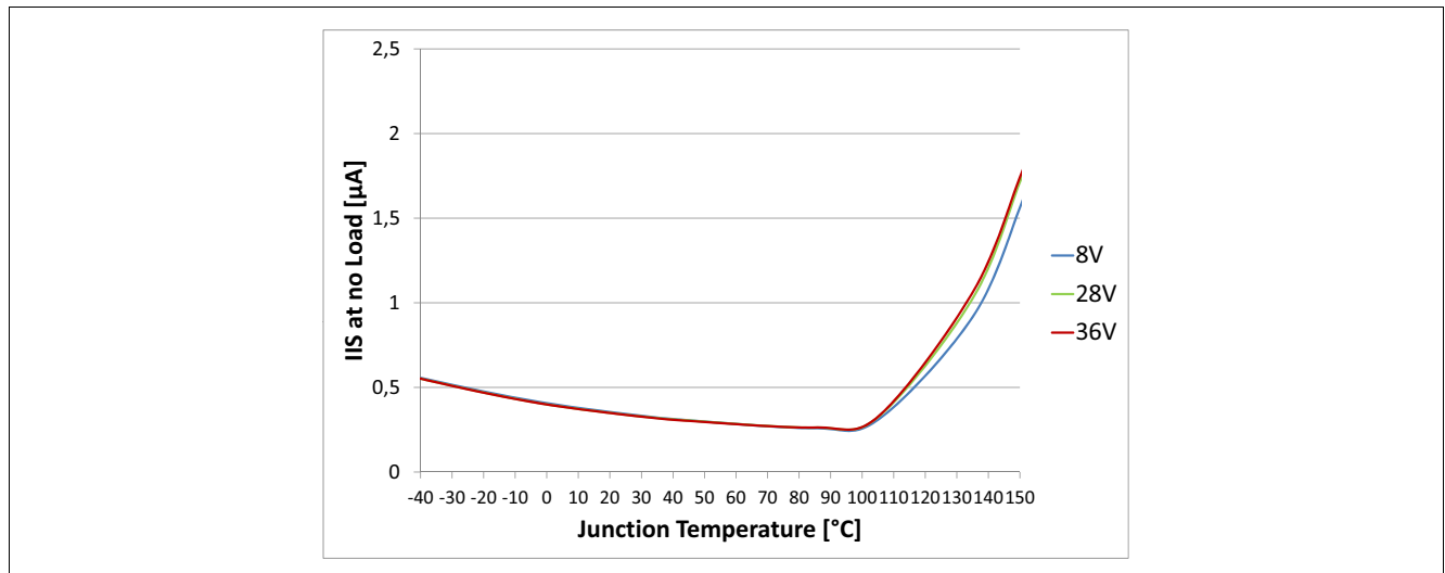
Figure 44 Current Sense at no Load I_{IS} = f(T_J; V_S) , I_L = 0 A
