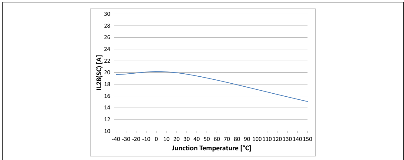
Figure 43 Overload Condition in the High Voltage Area I_{L28(SC)} = f(T_J; V_S)
