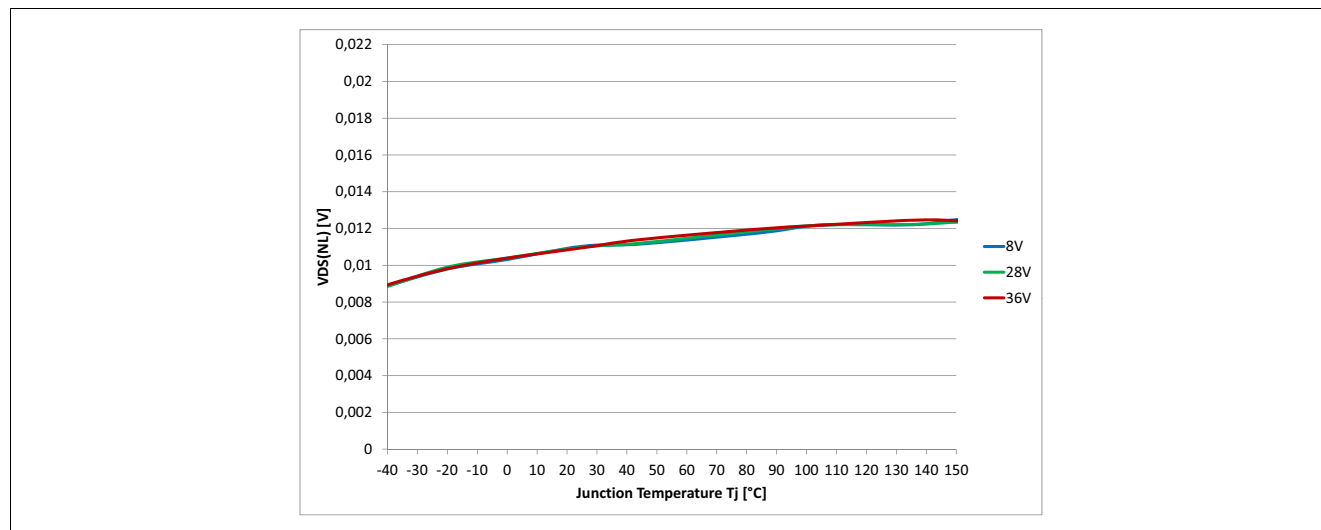
Figure 33 Output Voltage Drop Limitation at Low Load Current V_{DS(NL)} = f(T_J) and V_{DS(NL)} = f(V_G)
