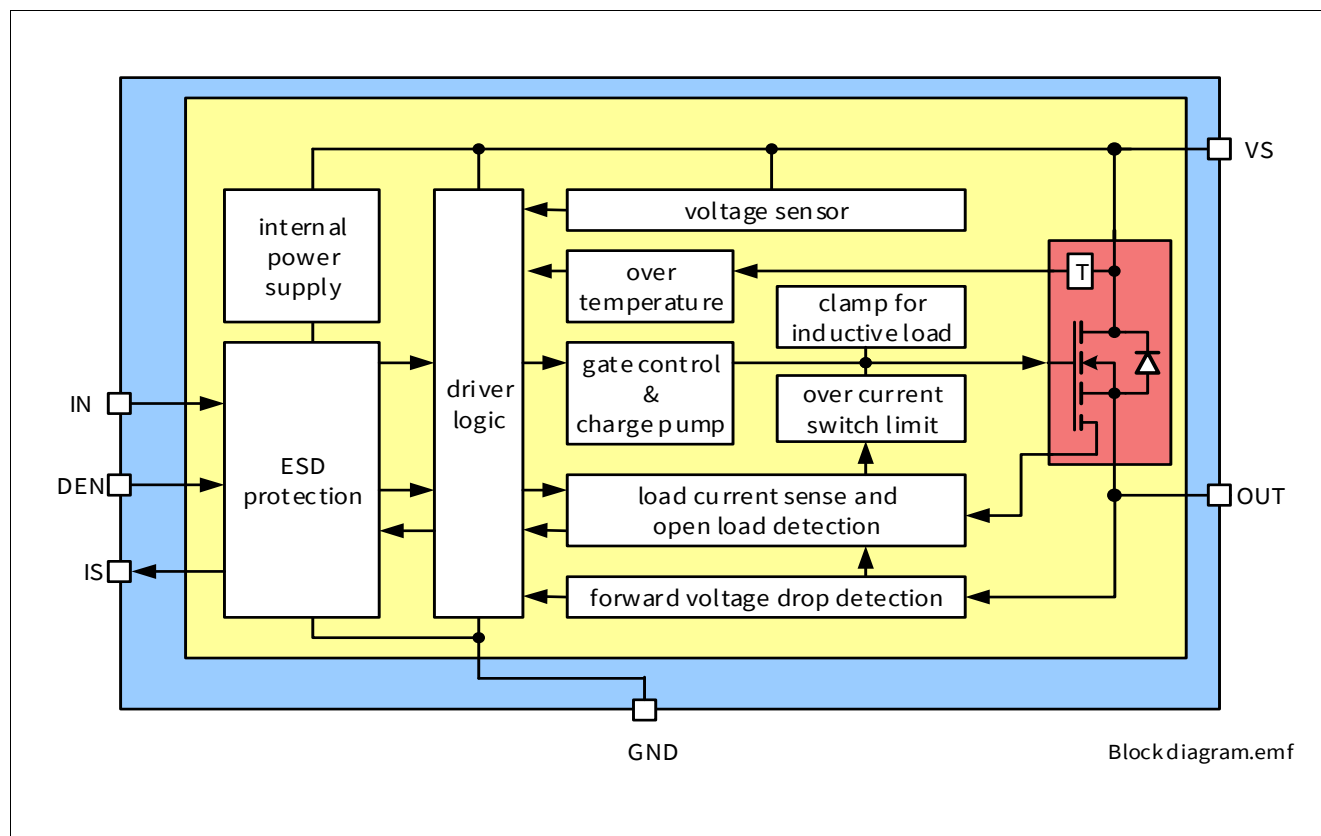
Figure 1 Block Diagram for the BTT6050-1ERA
