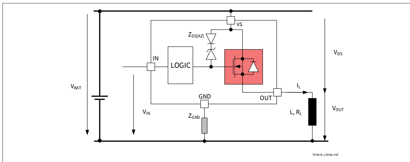
Figure 10 Output Clamp
