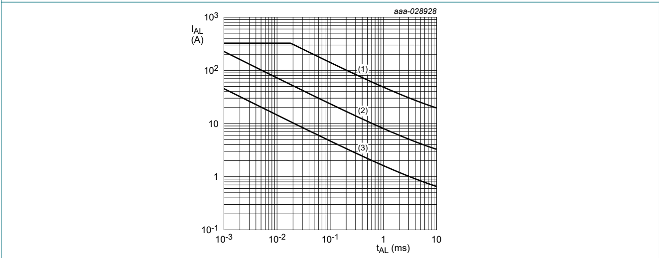
Fig. 5. Avalanche rating; avalanche current as a function of avalanche time
