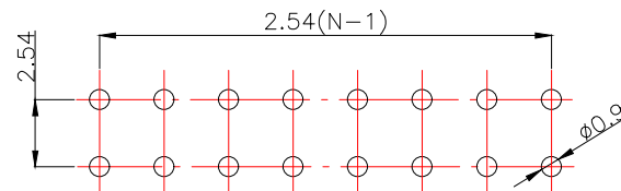
[P.C.B.LAYOUT]
