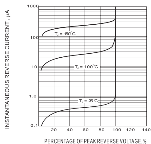
Fig.5-TYPICAL REVERSE CHARACTERISTIC
