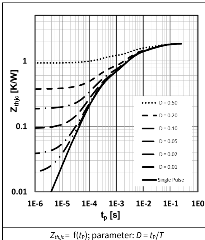
Figure 7 Max. transient thermal impedance
