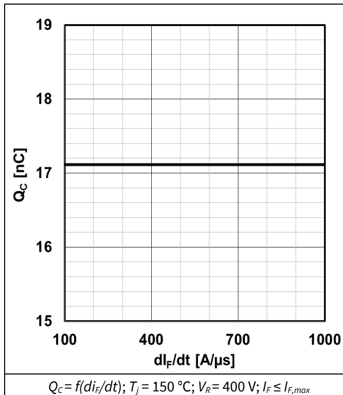
Figure 5 Typ. cap. charge vs. current slope
