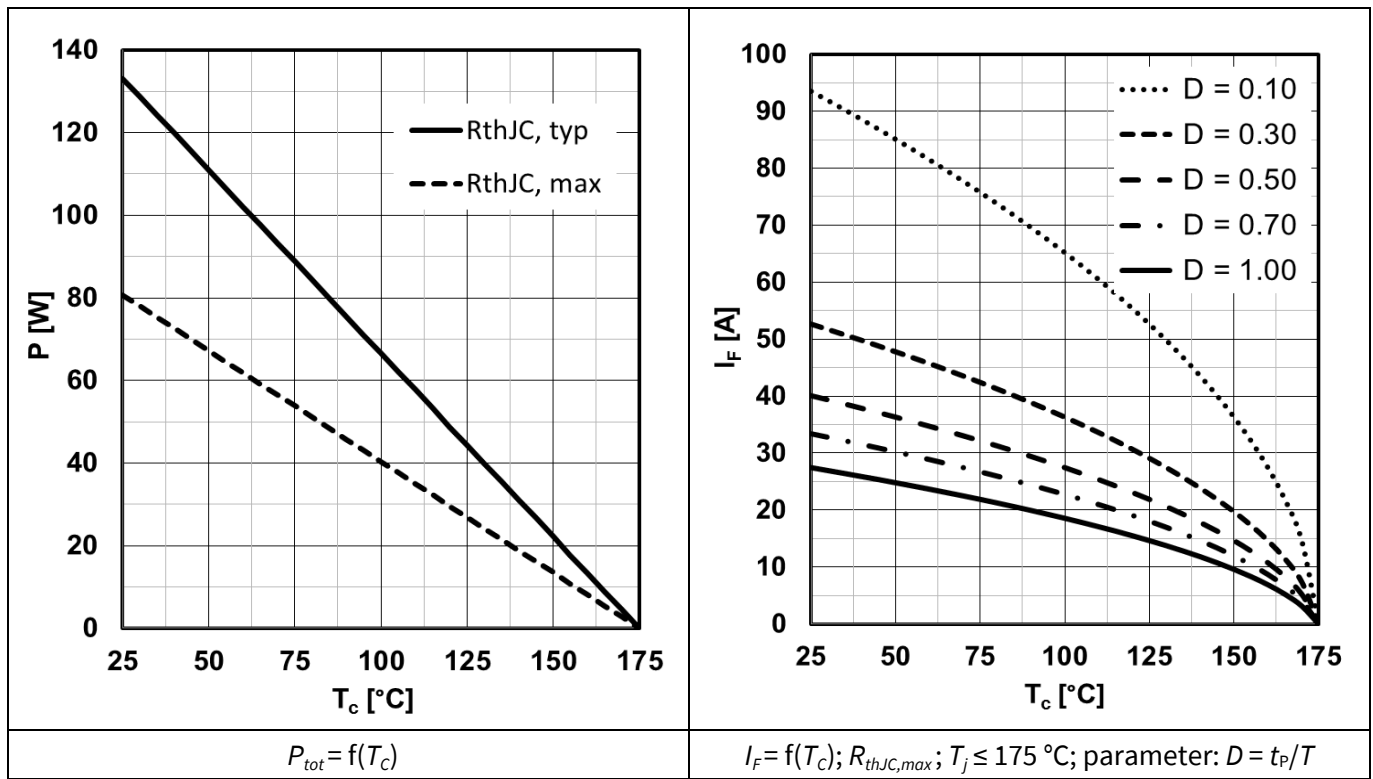
Figure 1 Power dissipation
