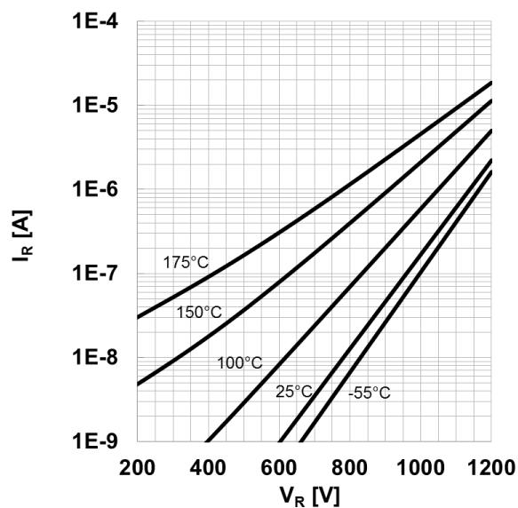
Figure 6. Typical reverse characteristics, I_R=f(V_R) , parameter: T_{vj}
