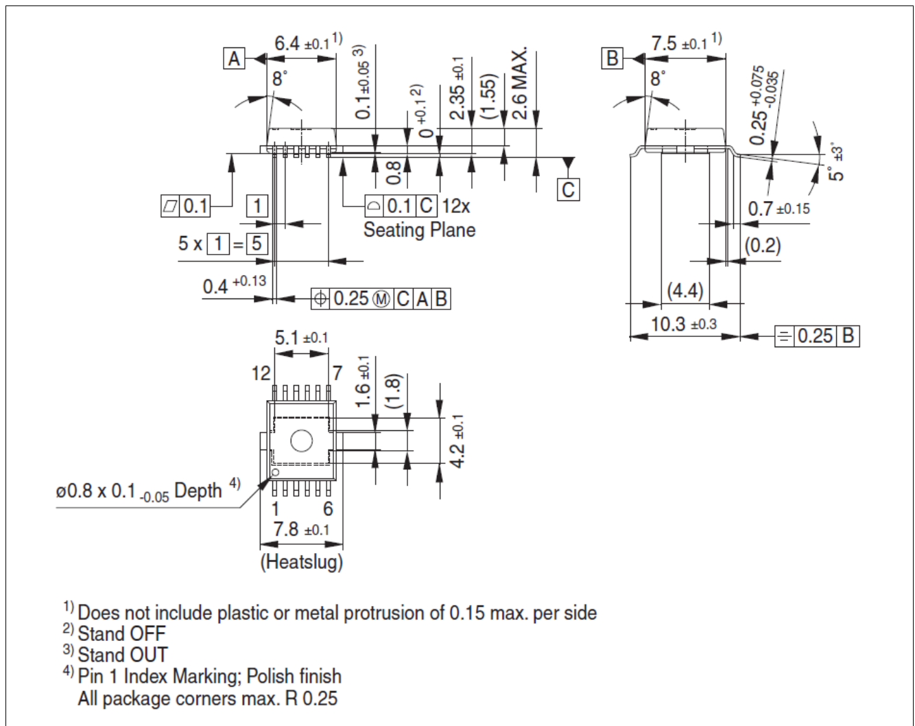
Figure 9 PG-DSO-12-17
