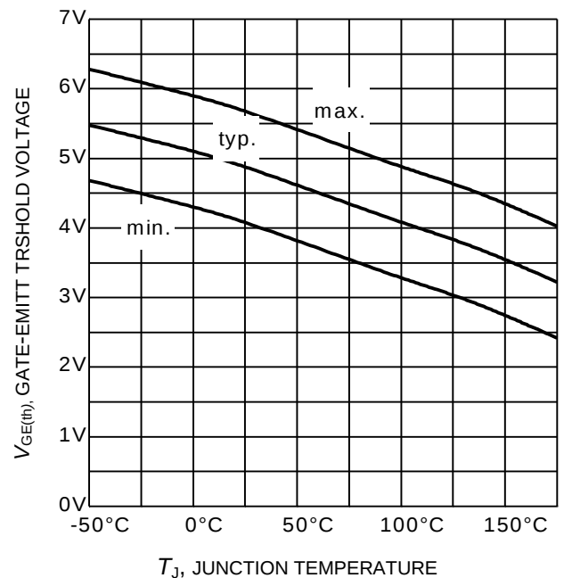
Figure 12. Gate-emitter threshold voltage as a function of junction temperature ( I_C = 60\text{ }\mu\text{A} )
