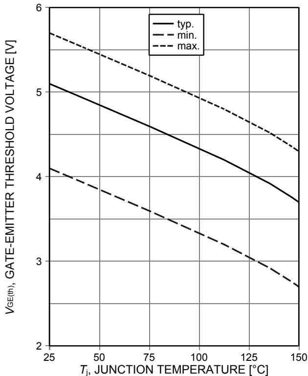
Figure 11. Gate-emitter threshold voltage as a function of junction temperature ( I_{\text{C}}=0.29\text{mA} )
