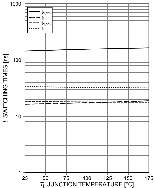
Figure 10. Typical switching times as a function of junction temperature (ind. load, V_{\text{CE}}=400\text{V} , V_{\text{GE}}=0/15\text{V} , I_{\text{C}}=30\text{A} , r_{\text{G}}=10\Omega , test circuit in Fig. E)
