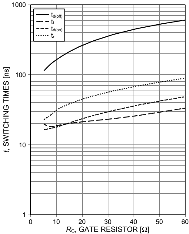
Figure 9. Typical switching times as a function of gate resistor (ind. load, T_j=175^{\circ}\text{C} , V_{\text{CE}}=400\text{V} , V_{\text{GE}}=0/15\text{V} , I_{\text{C}}=30\text{A} , test circuit in Fig. E)
