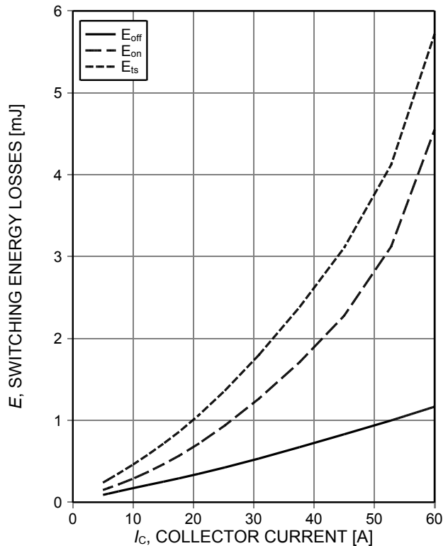
Figure 12. Typical switching energy losses as a function of collector current (ind. load, T_j=175^{\circ}\text{C} , V_{\text{CE}}=400\text{V} , V_{\text{GE}}=0/15\text{V} , R_{\text{G}}=10\Omega , test circuit in Fig. E)
