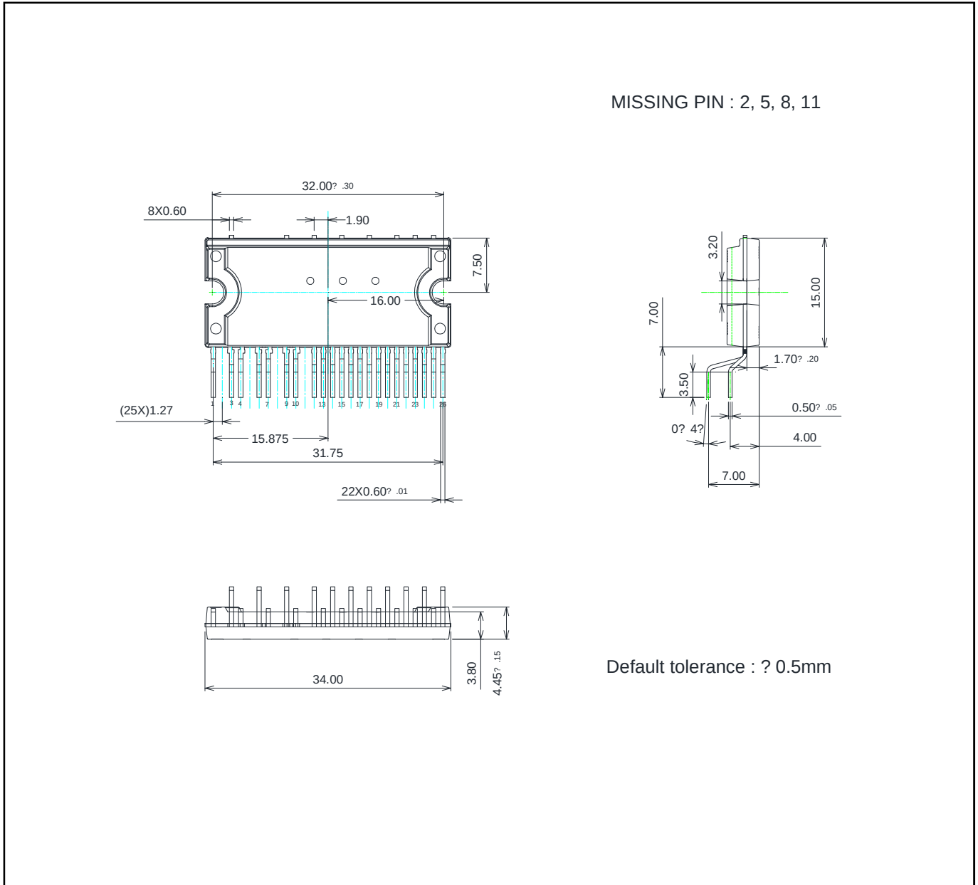
Figure 18 IM393-M6F
