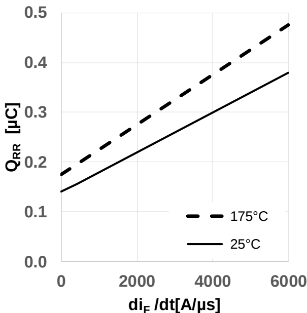
Figure 19 Typical reverse recovery charge as a function of diode current slope (Q_{rr} = f(di_i/dt), V_{DD} = 800V, V_{GS} = 0V/18V, I_D = 13A, \text{ind. load, test circuit in Fig. E, body diode at } V_{GS} = 0V)
