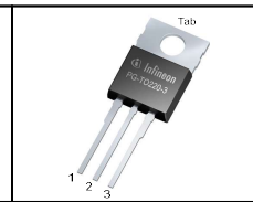
PG-TO220-3-1
