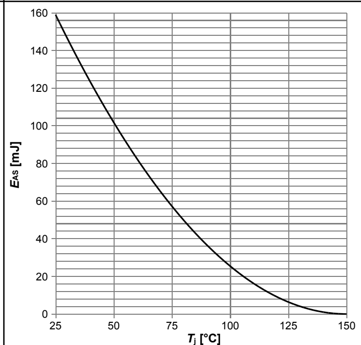
Diagram 12: Avalanche energy
