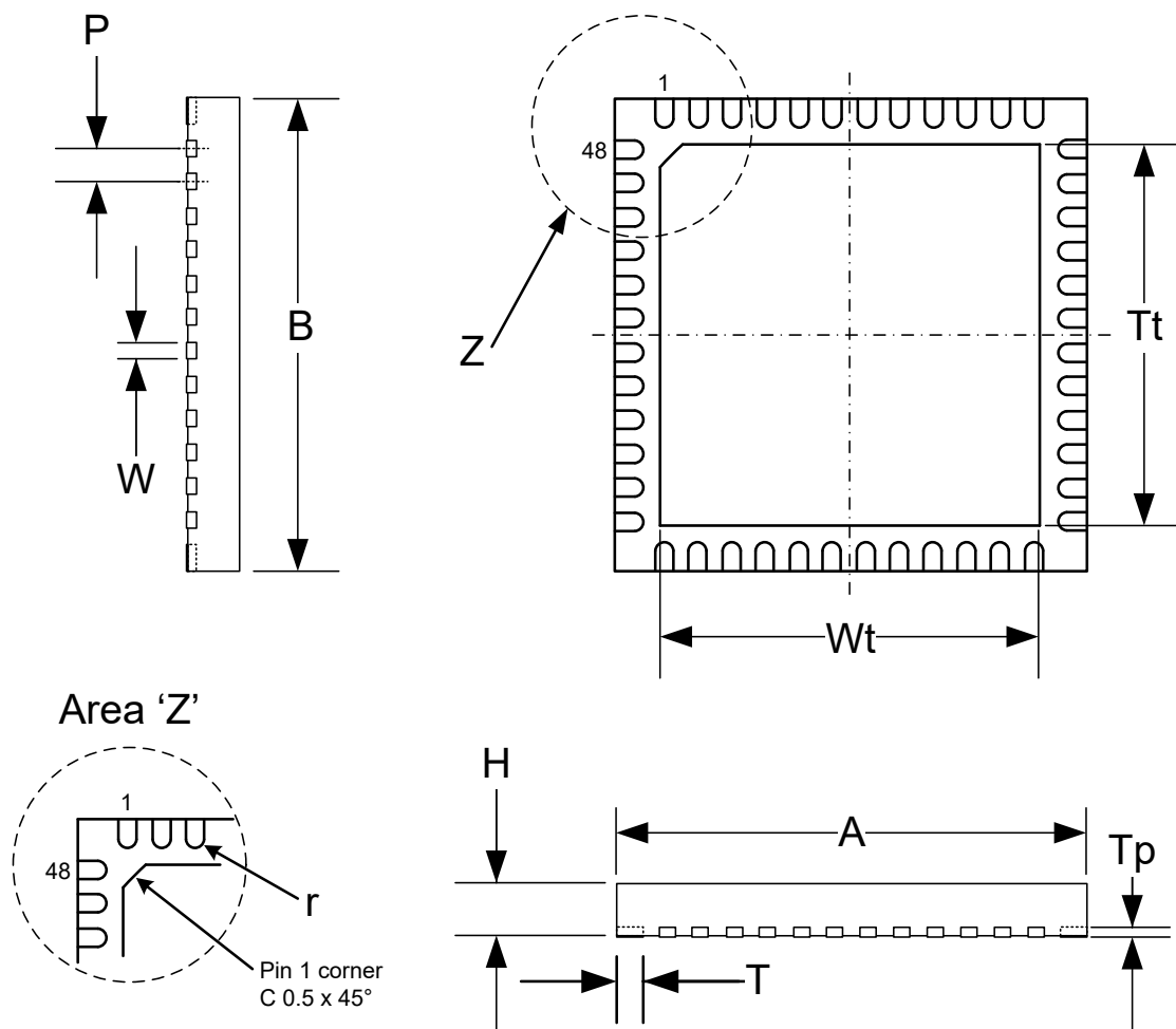
Figure 11.1 QFN(7x7)-48 Package
